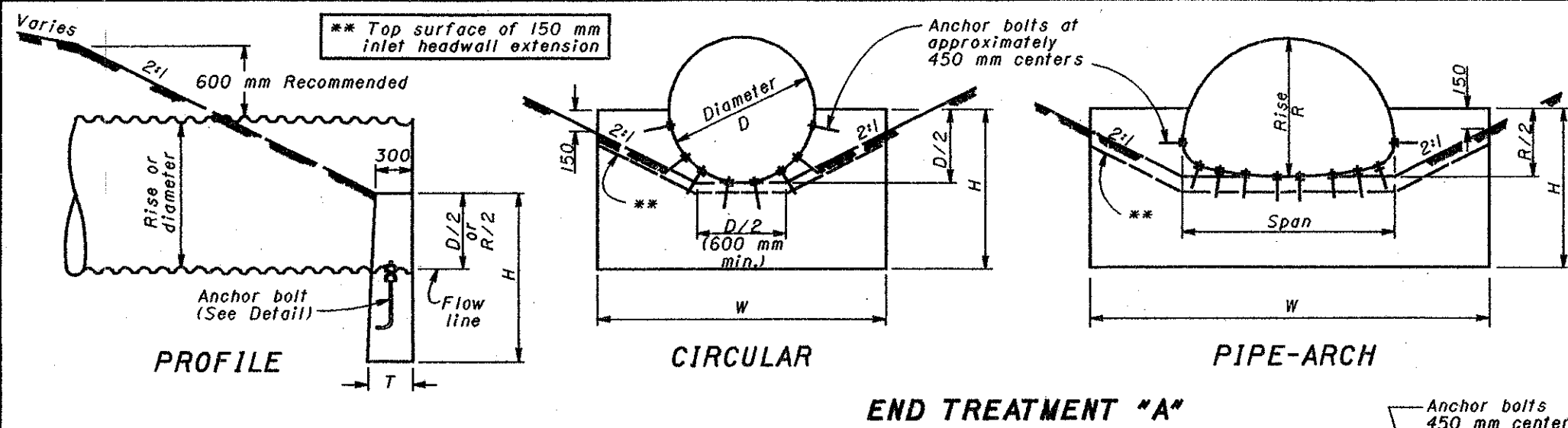
HEADWALL FOR CORRUGATED METAL PIPE & PLASTIC PIPE
