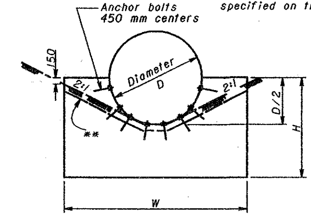
HEADWALL FOR CORRUGATED METAL PIPE & PLASTIC PIPE
