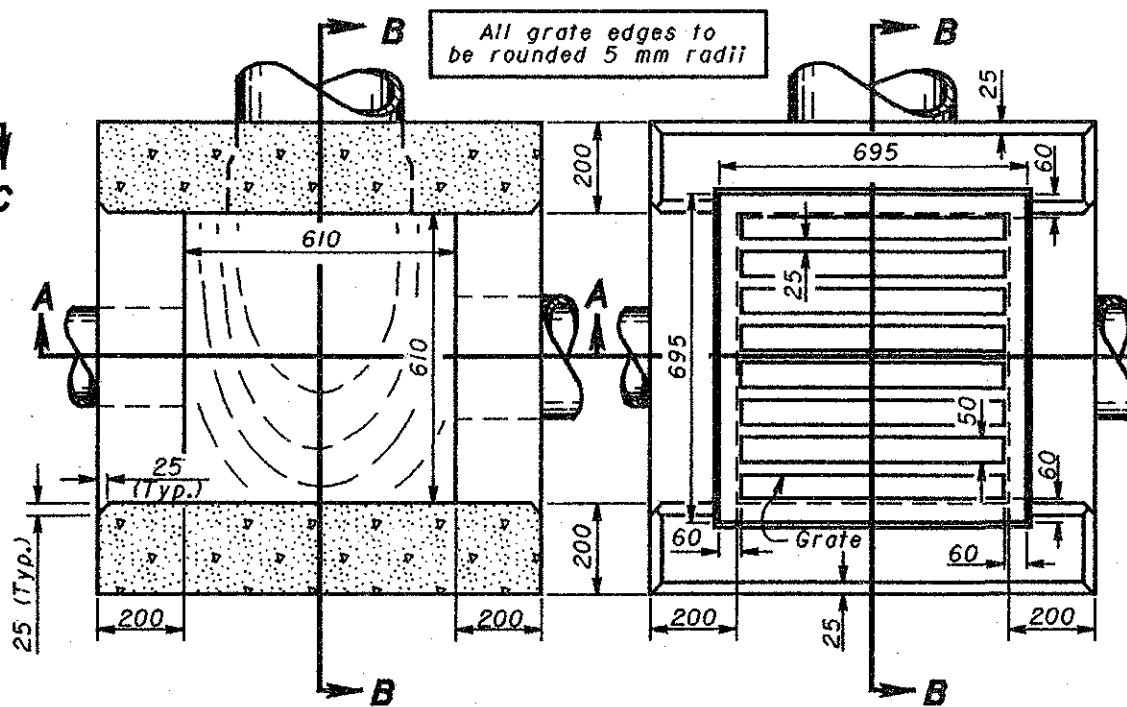
SECTION C-C
