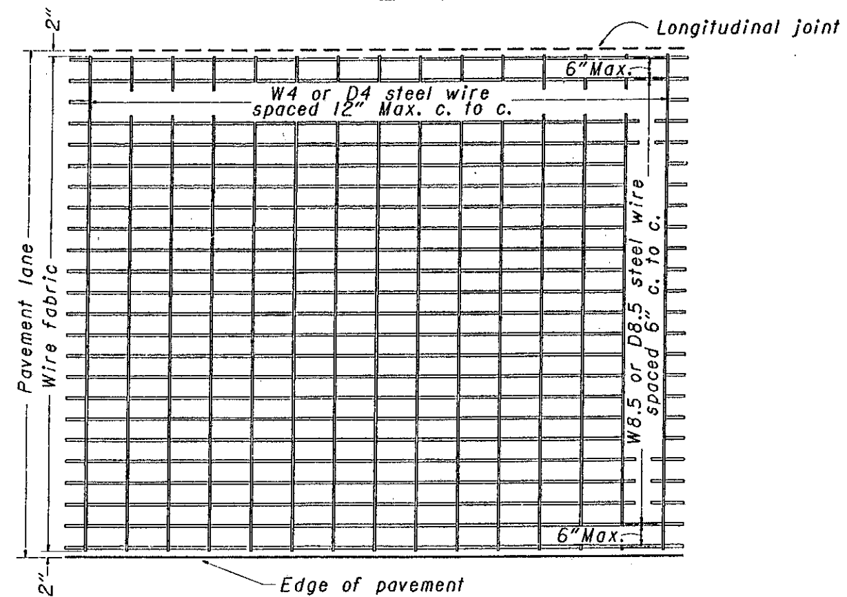
WIRE FABRIC DETAIL
