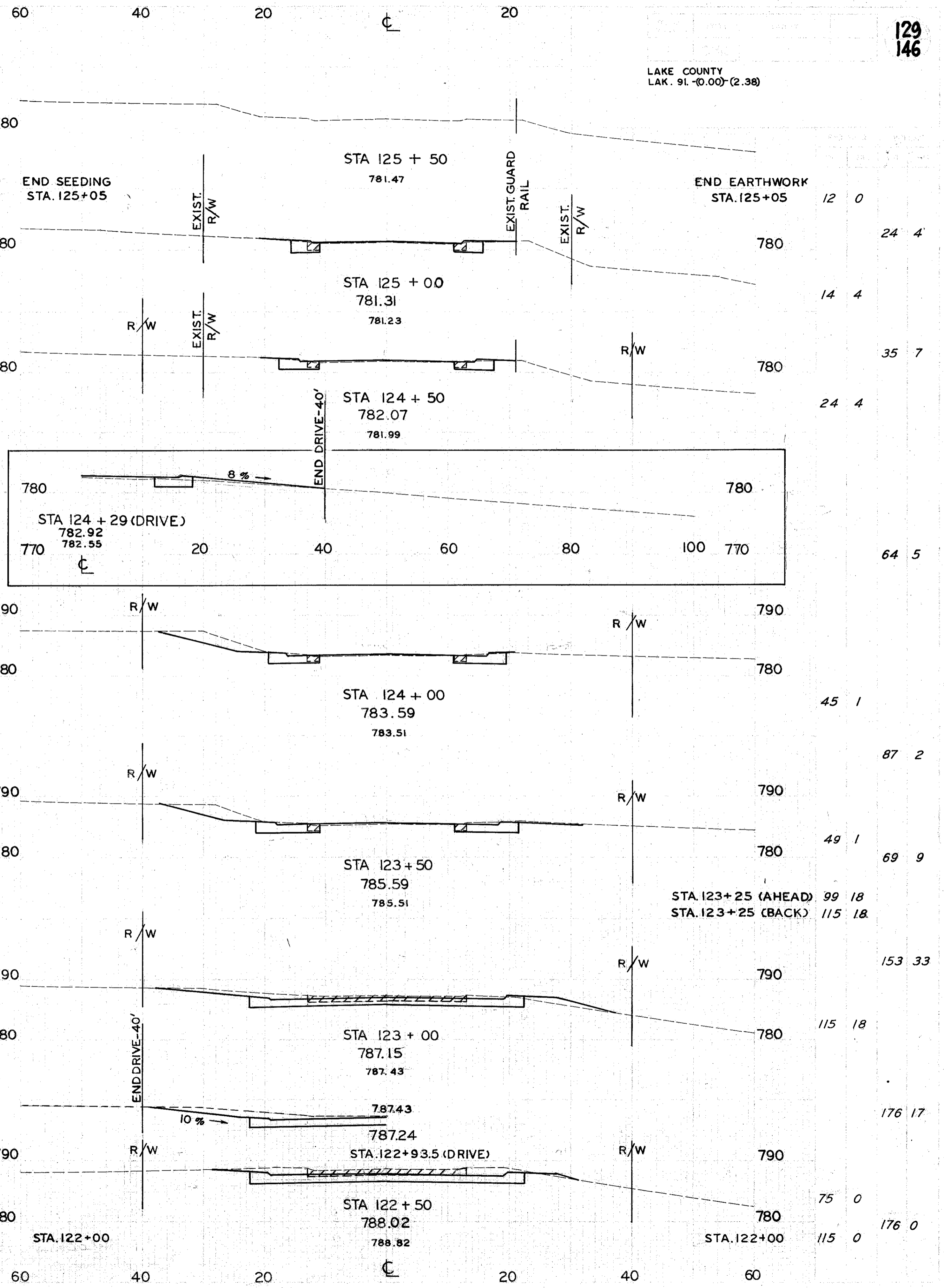
CROSS SECTIONS . . . SR.84 . . . STA 116 + 50 TO STA 125 + 50
