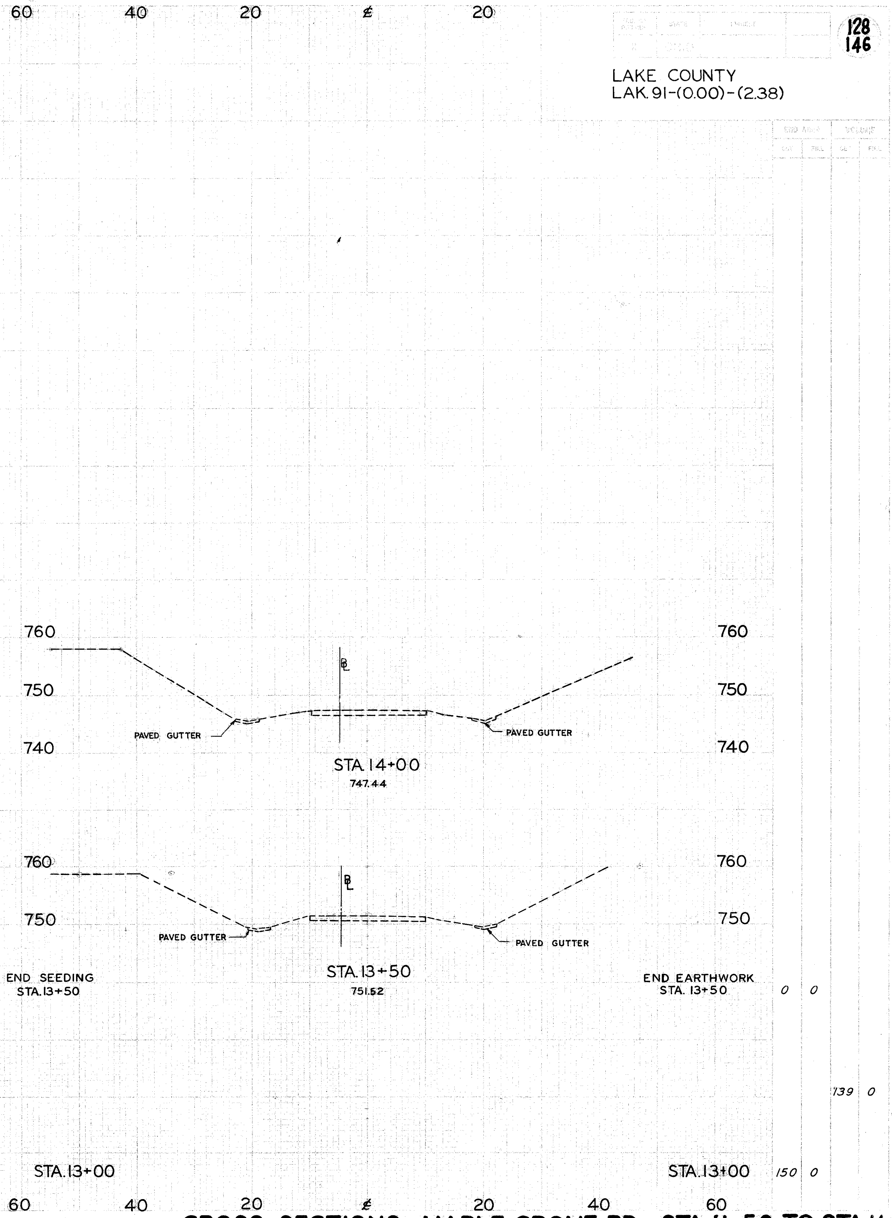
CROSS SECTIONS...MAPLE GROVE RD...STA.11+50 TO STA.14+00
