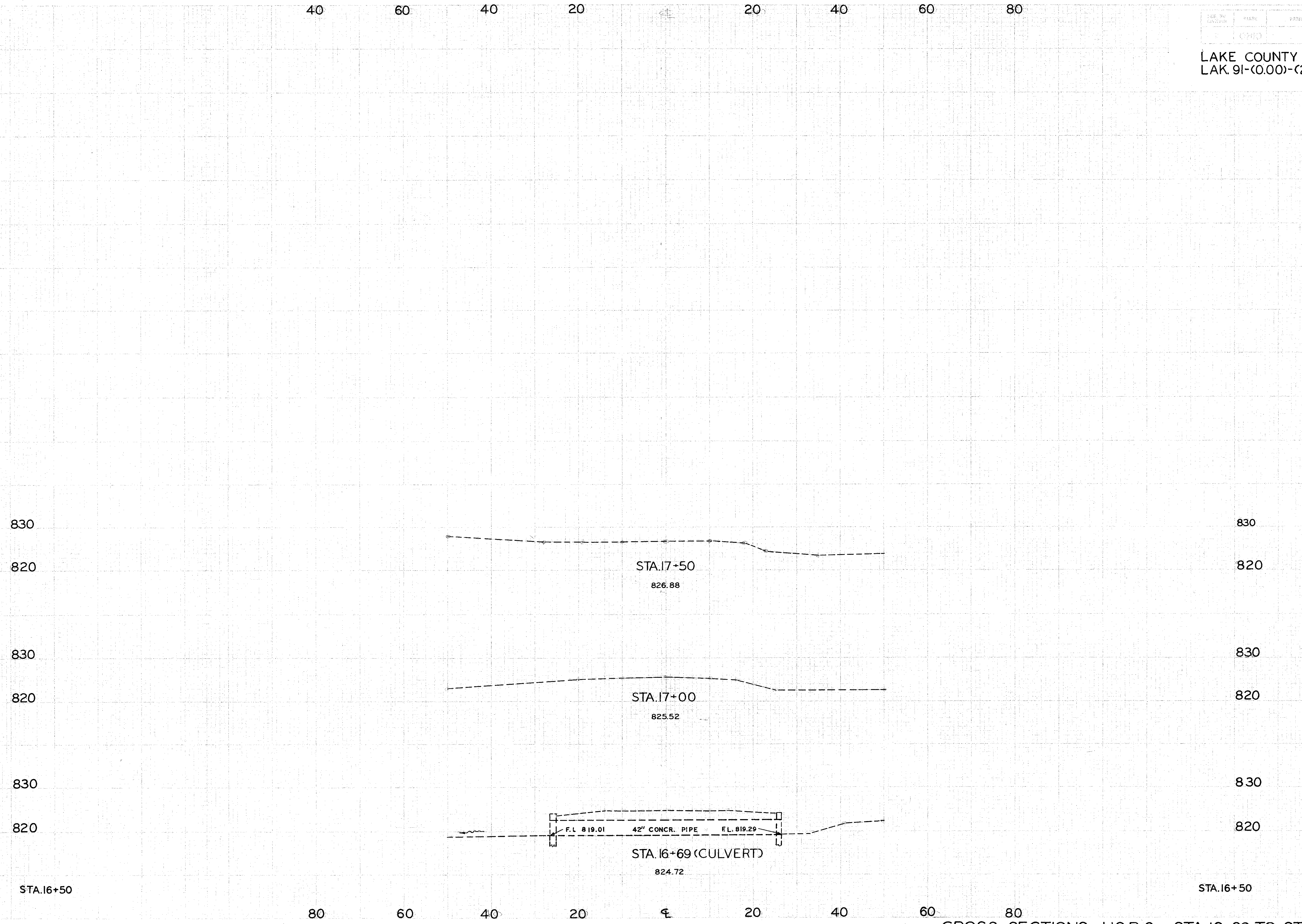
CROSS SECTIONS U.S.R.6 STA.16+69 TO STA.17+50
