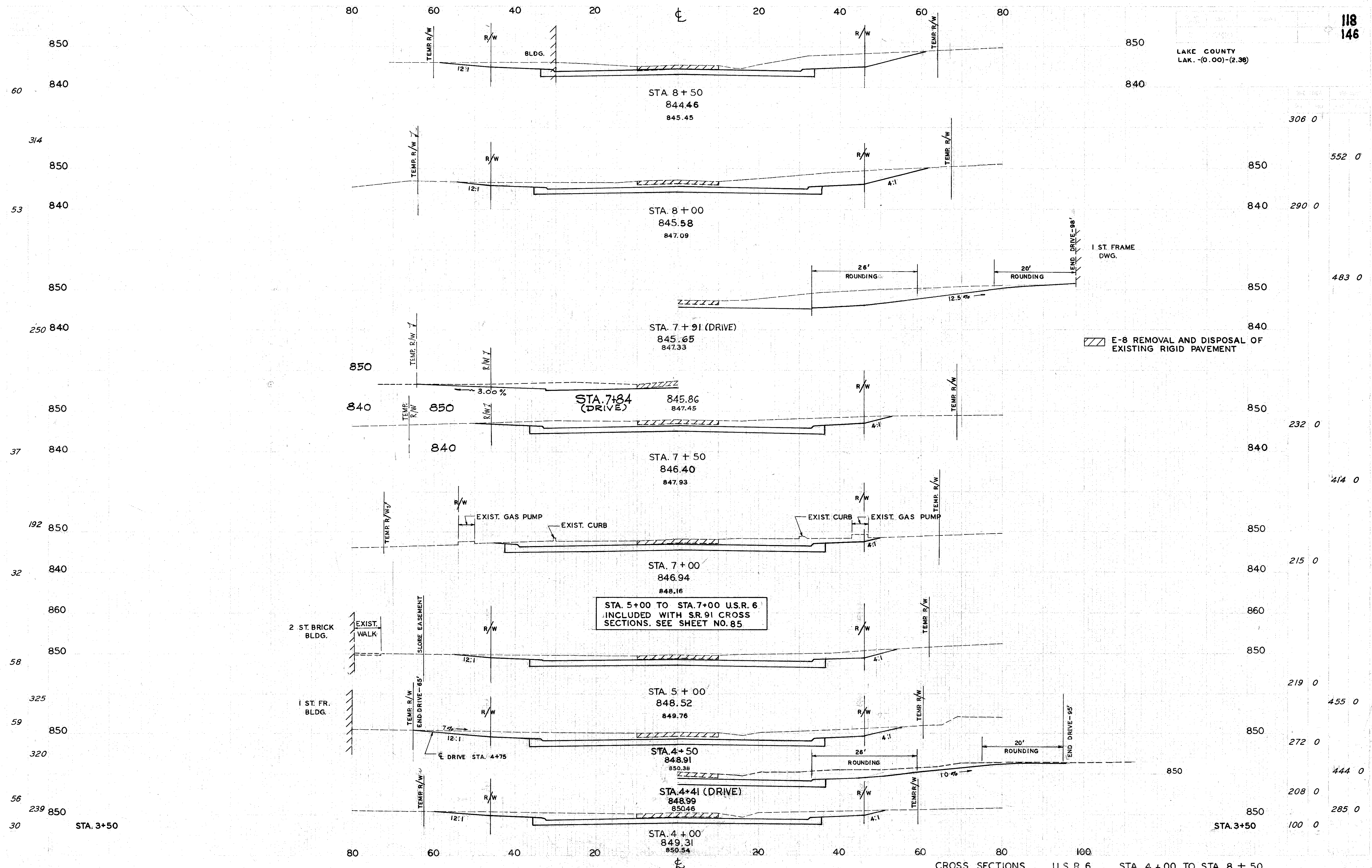
CROSS SECTIONS . . . U.S.R. 6 . . . STA 4 + 00 TO STA 8 + 50
