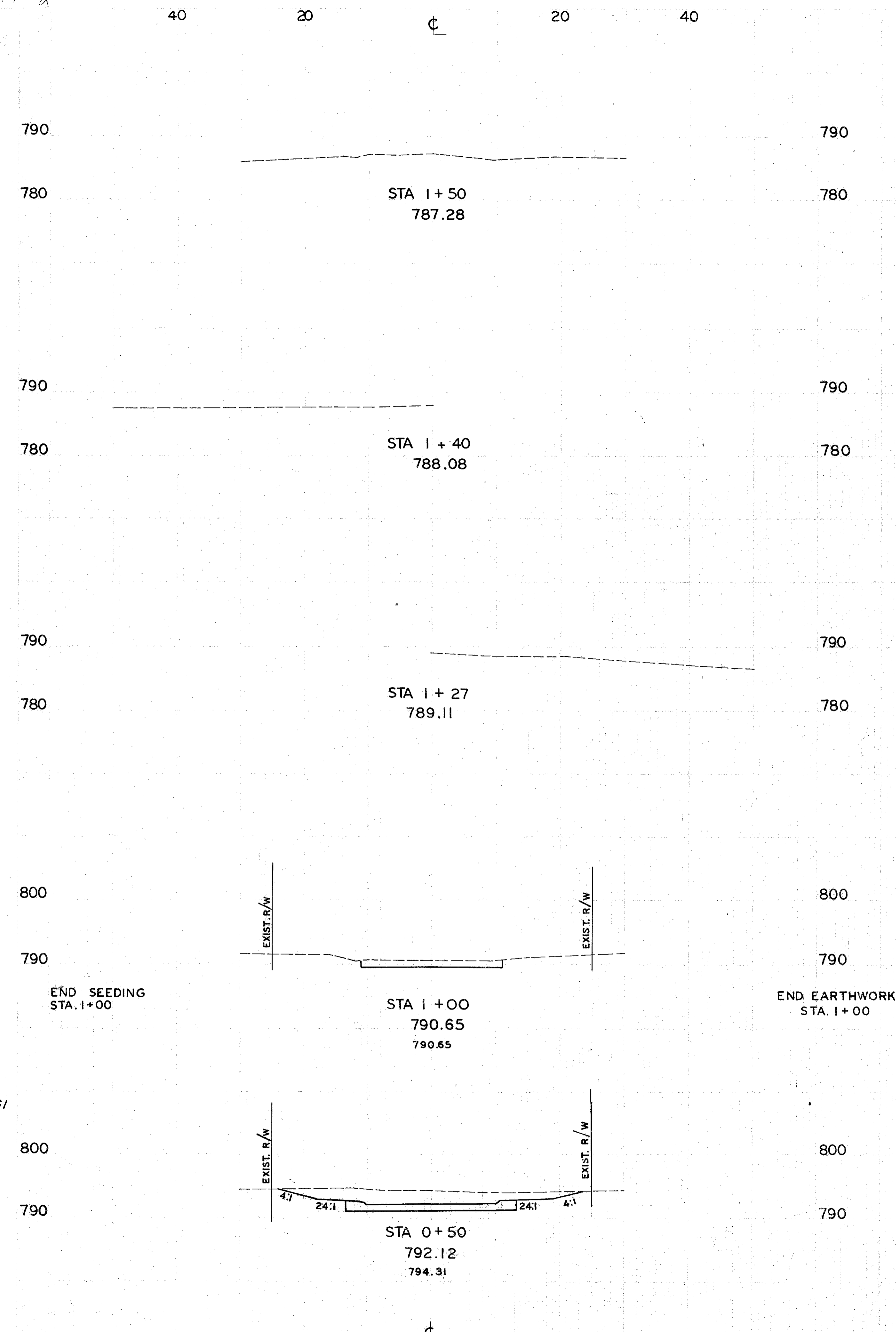
CROSS SECTIONS . . . TIMBERLINE DRIVE . . . STA 0+50 TO STA 1+50
