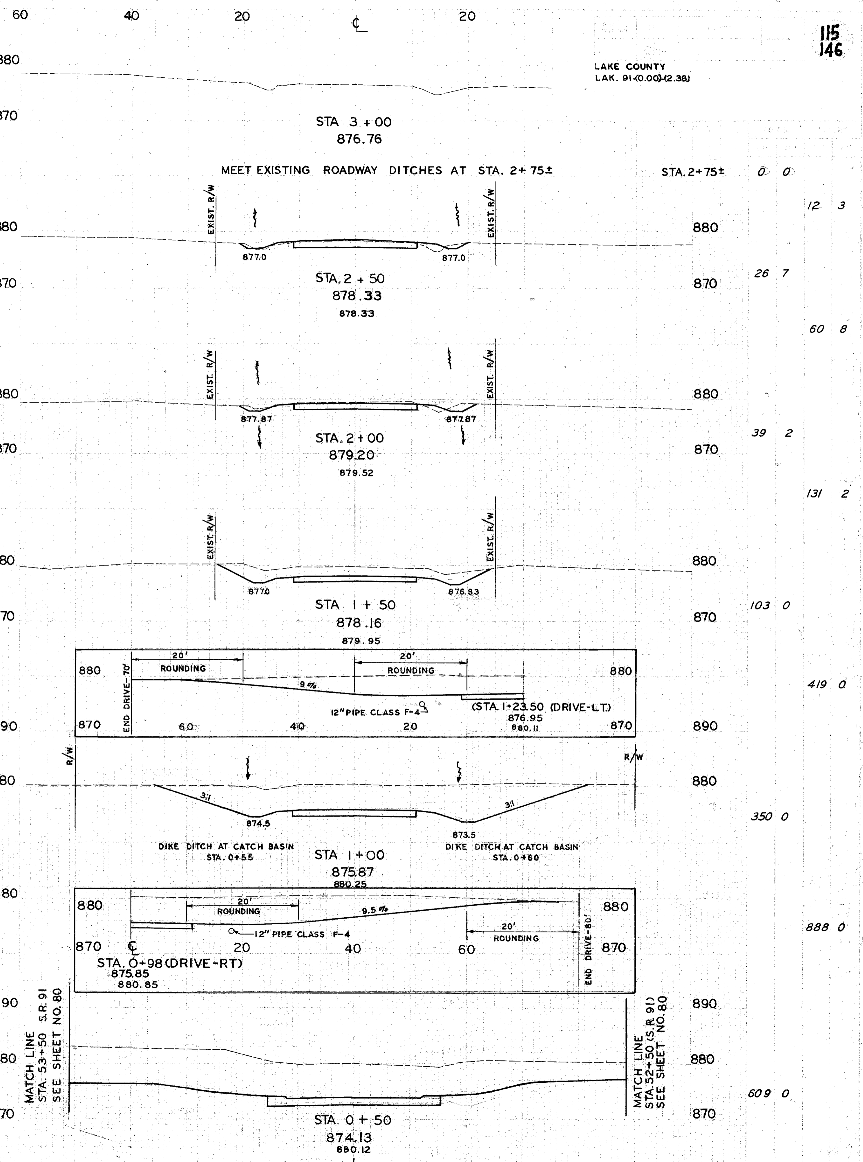
CROSS SECTIONS . . . DIXON ROAD . . . STA 0+50 TO STA 3+00
