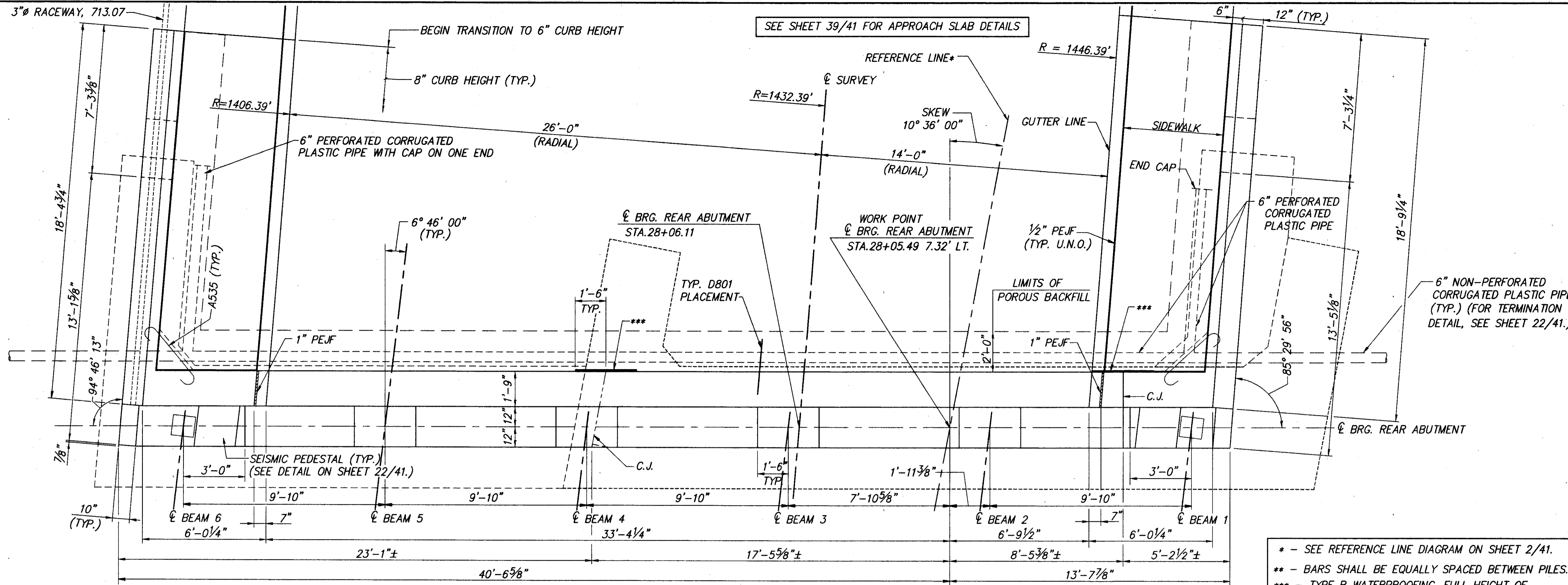
REAR ABUTMENT PLAN
