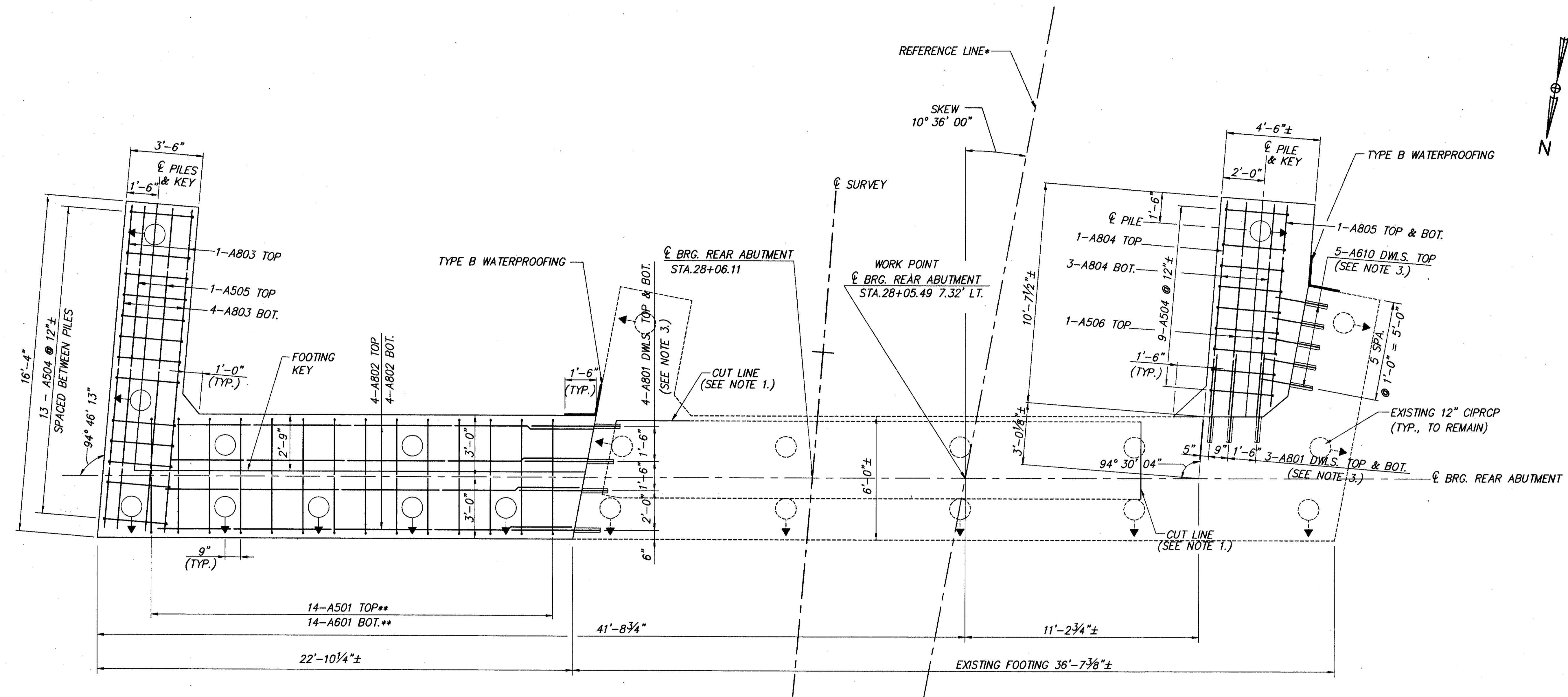
REAR ABUTMENT FOOTING PLAN
