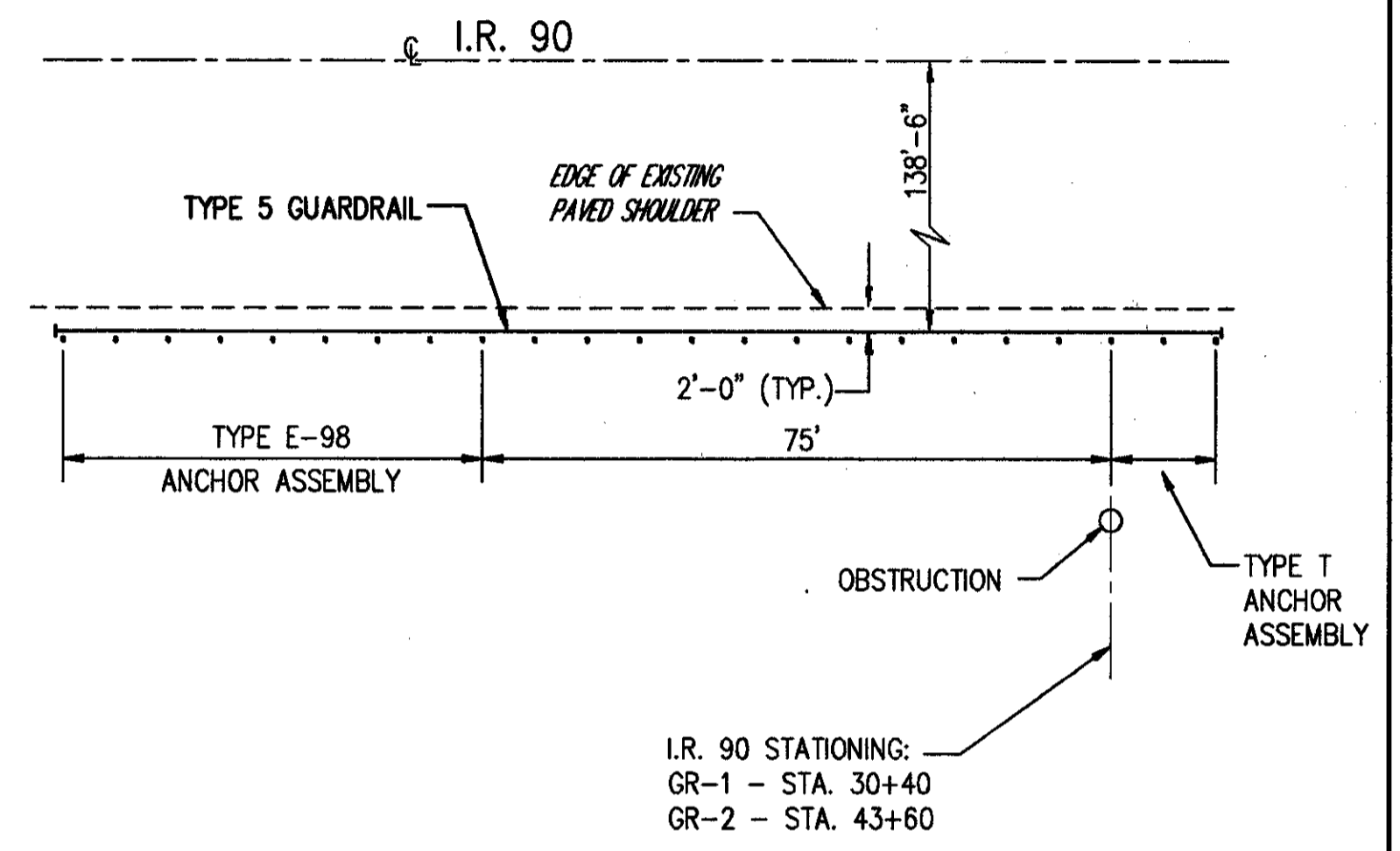
TYPICAL GUARDRAIL PLACEMENT DETAIL
