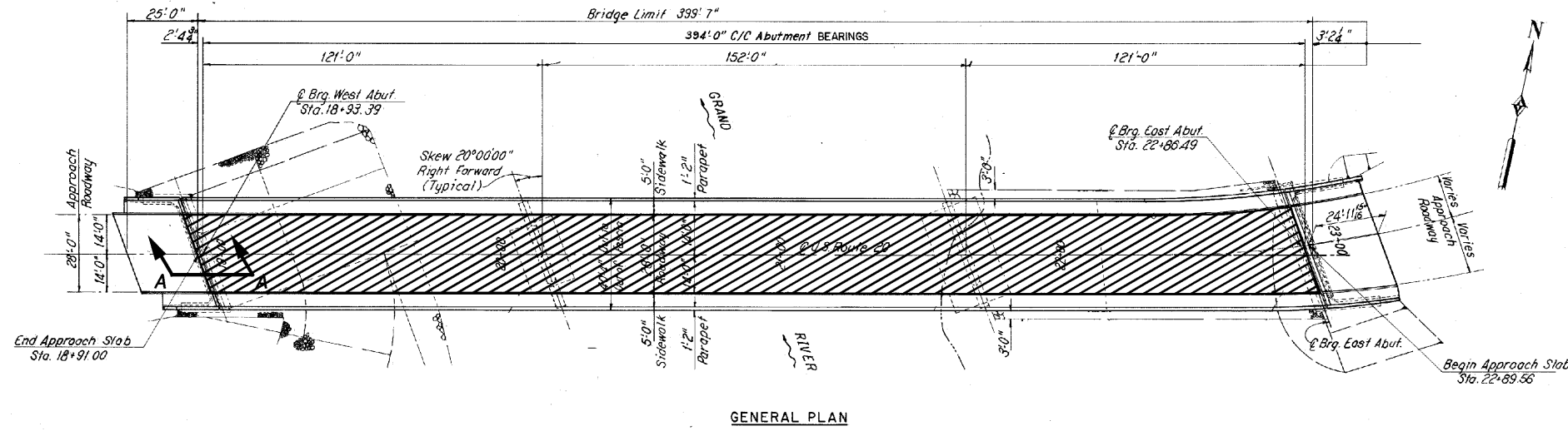
GENERAL PLAN
