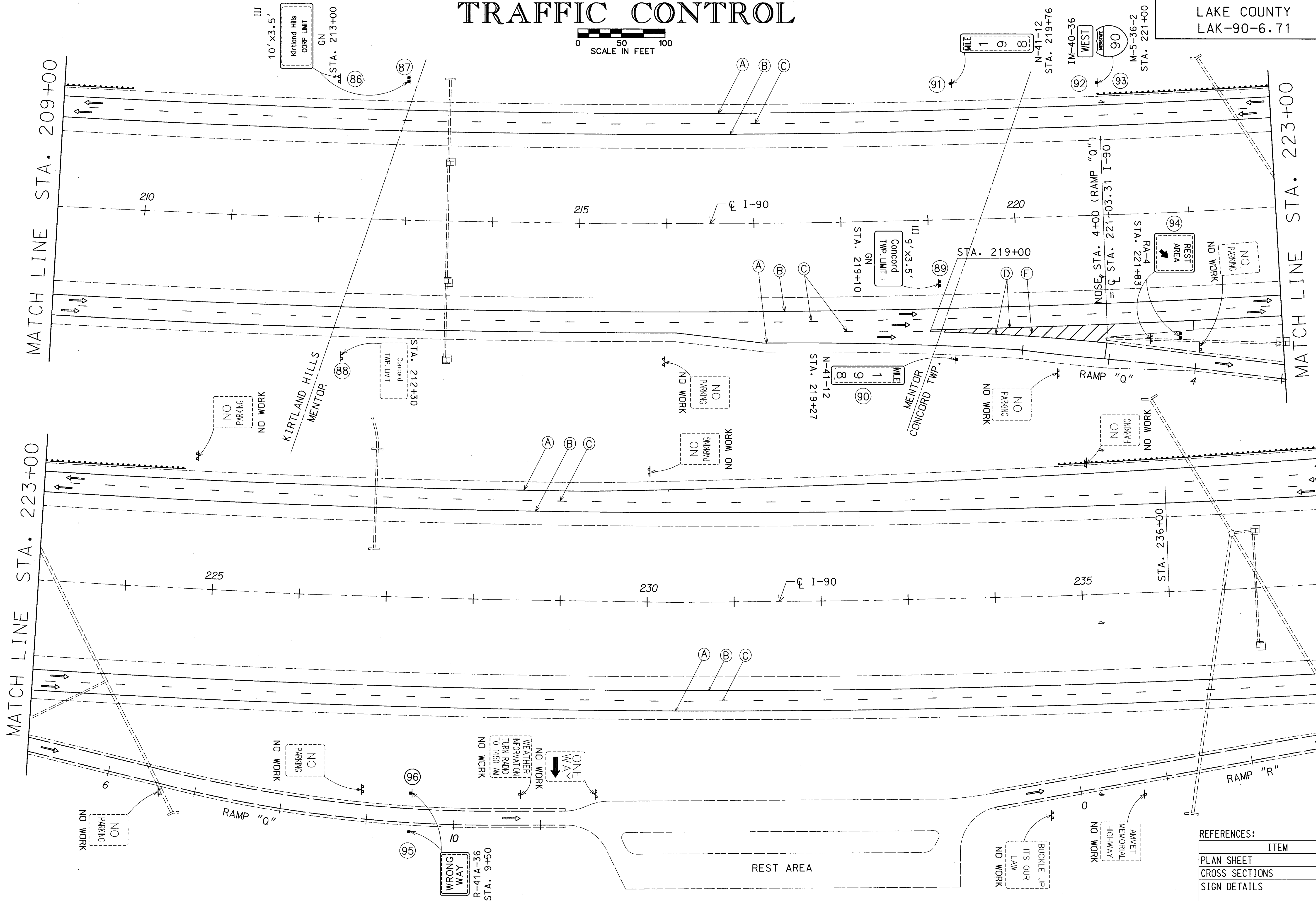
I-90 TRAFFIC CONTROL PLAN STA. 209+00 TO STA. 238+00
