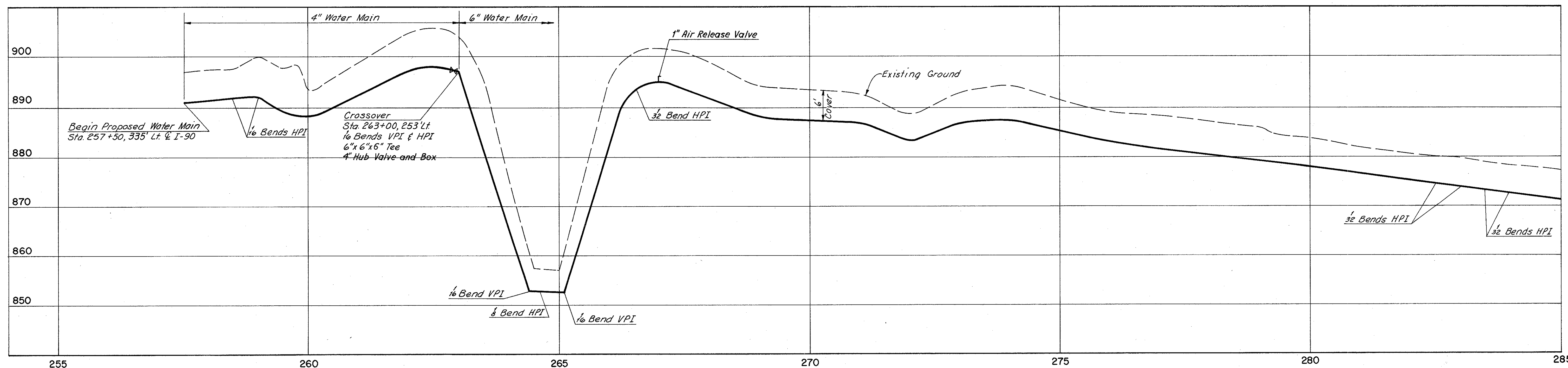
4" AND 6" WATER MAINS NORTH SIDE I-90
