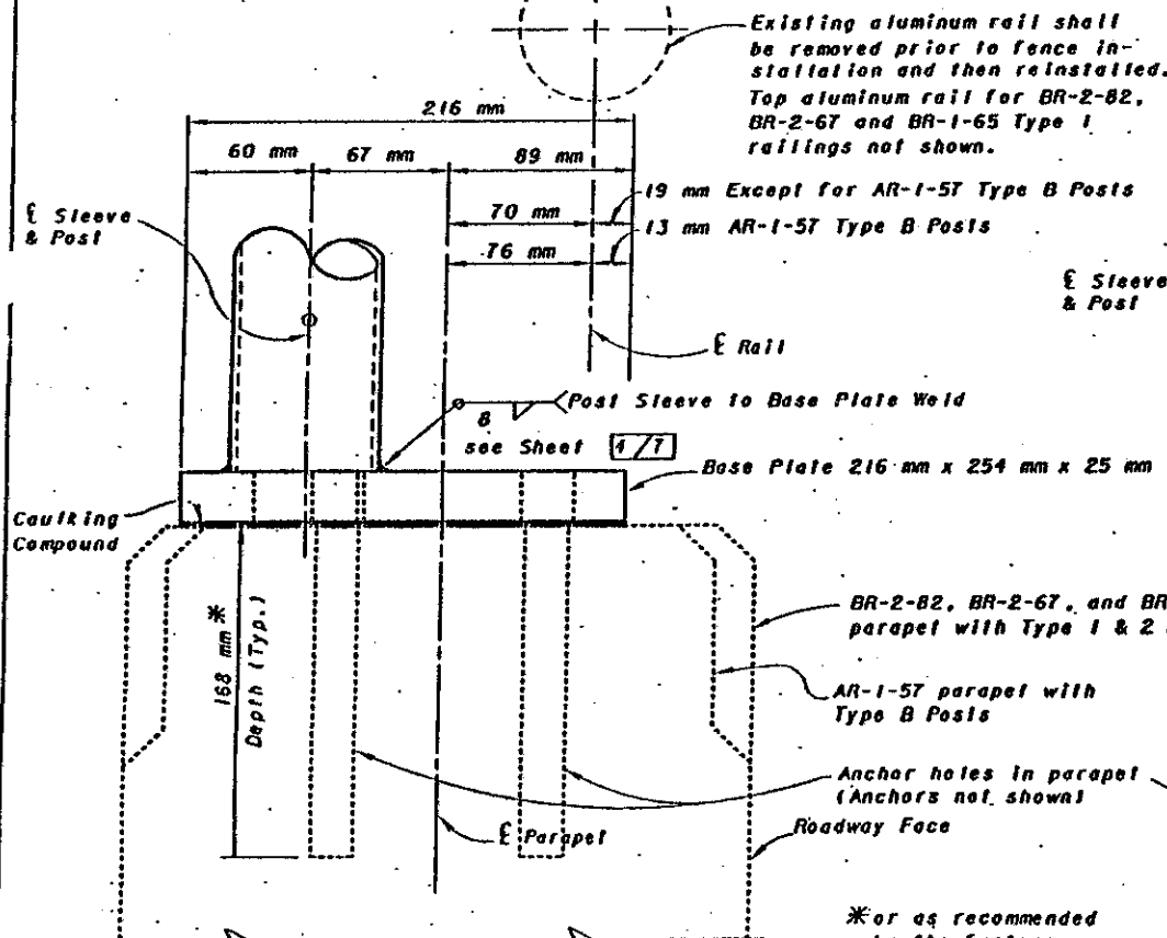
END VIEW BP-1
