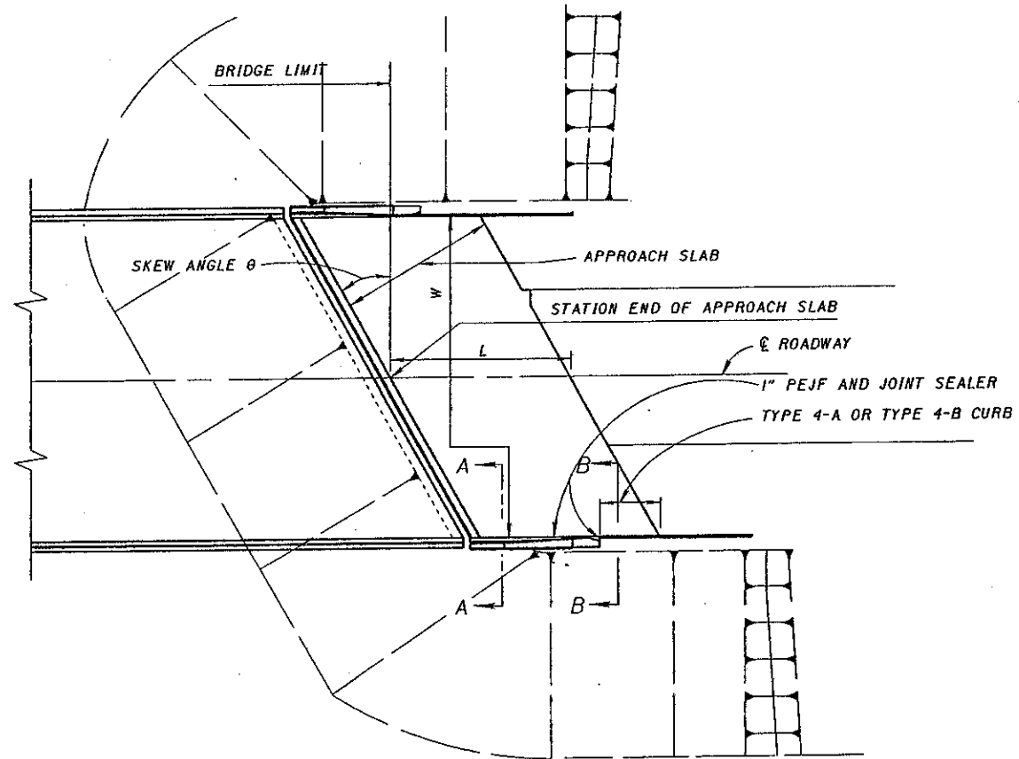
PLAN BRIDGE WITH DEFLECTOR PARAPETS
