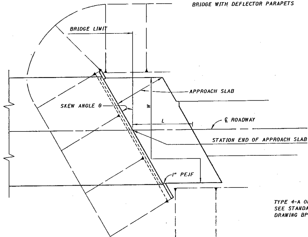
PLAN BRIDGE WITHOUT CURBS
