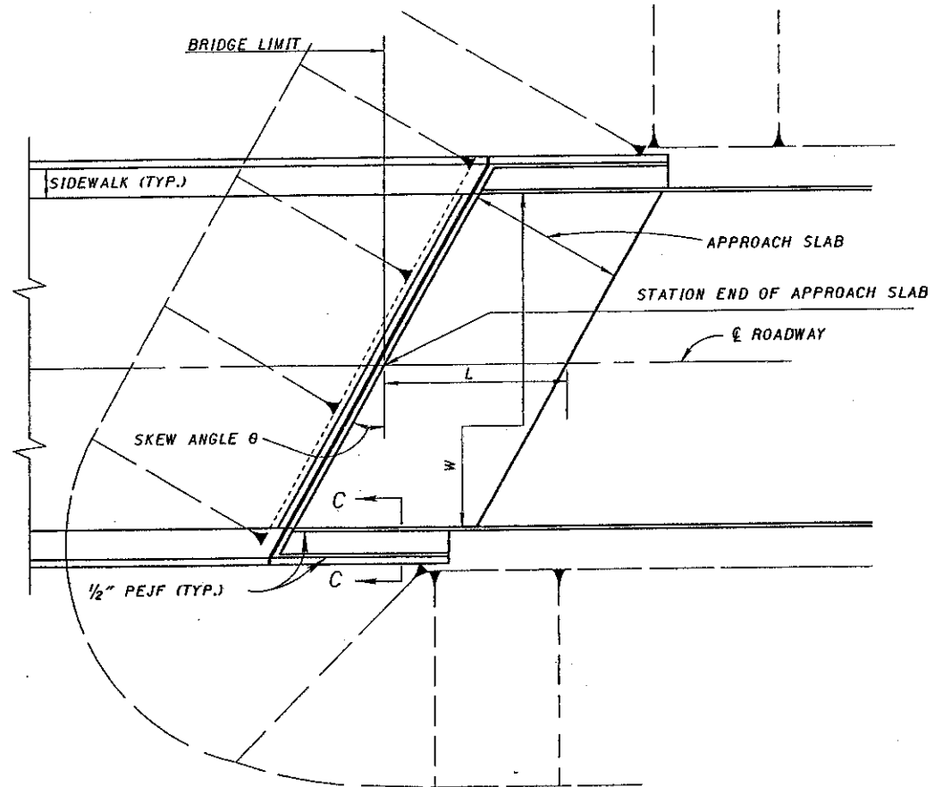
PLAN BRIDGE WITH SIDEWALKS
