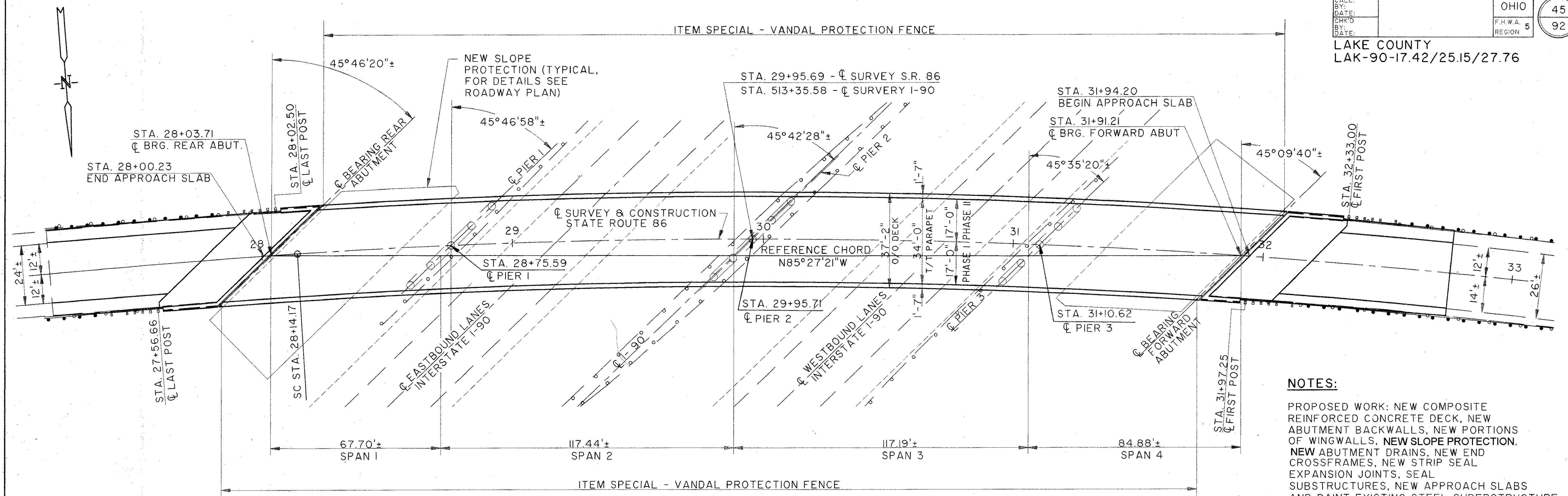
GENERAL PLAN
