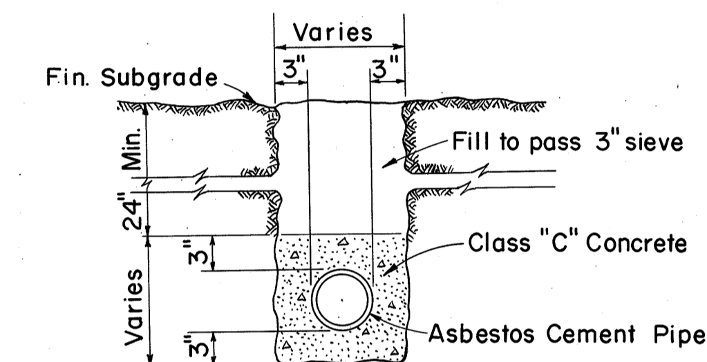
ONE WAY DUCT SECTION
