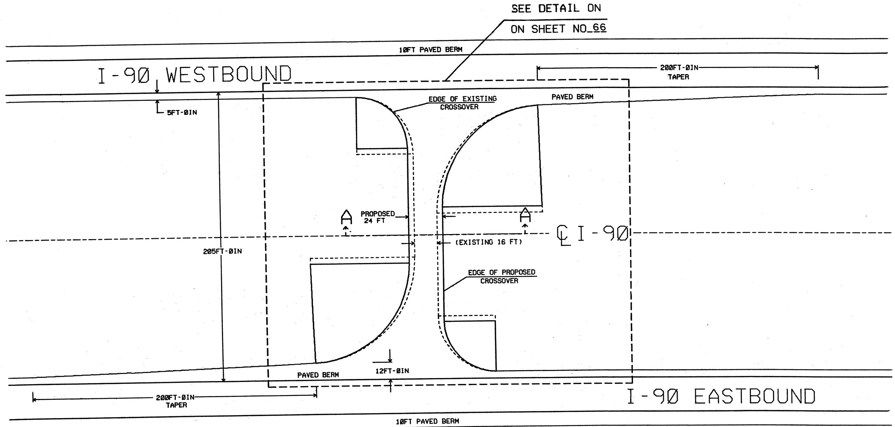
TYPICAL CROSSOVER WIDENING
