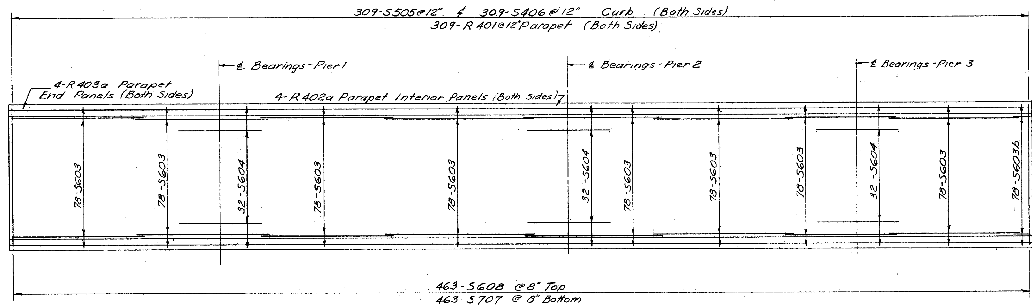
DECK REINFORCEMENT PLAN-WEST BRIDGE
