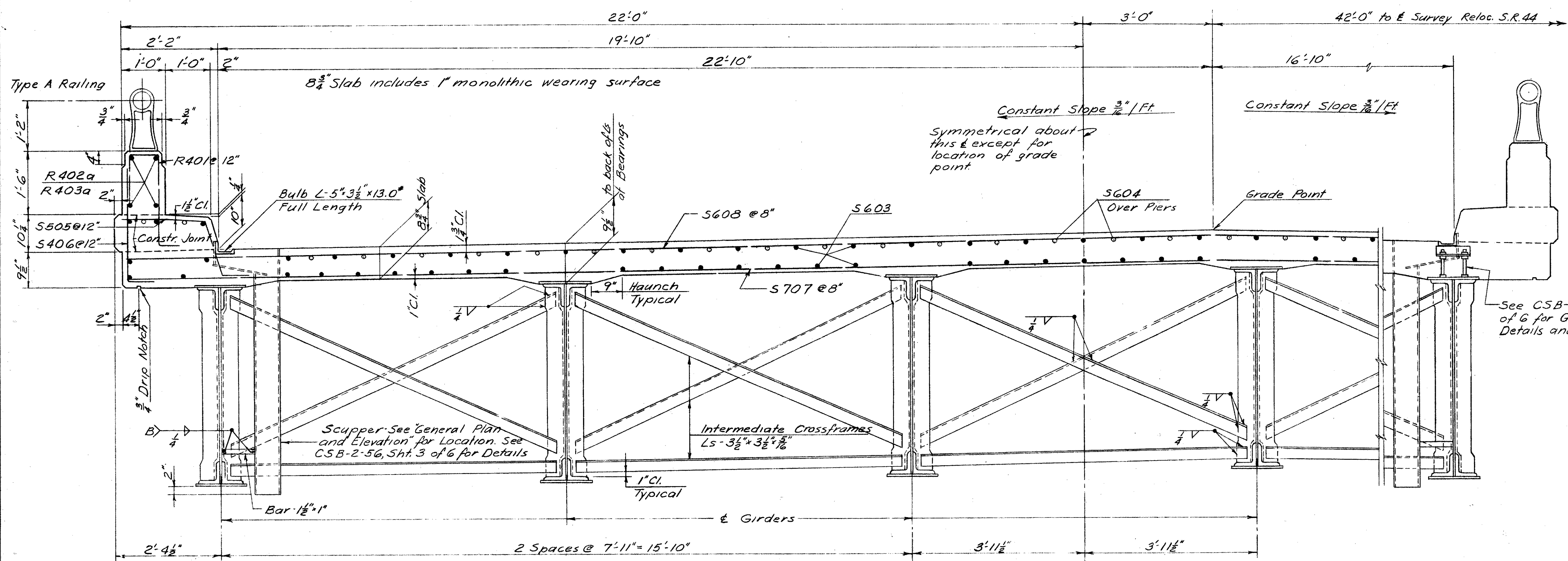
TYPICAL HALF SECTION-WEST BRIDGE
