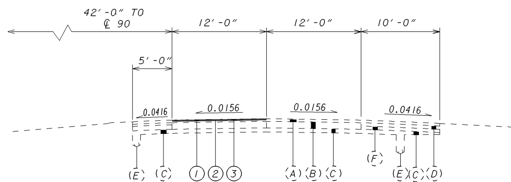
2 LANE NORMAL SECTION SLM 14.63 TO 19.62 SLM 20.57 TO 29.88 (FOR LEFT LANES MIRROR ABOUT CL)
