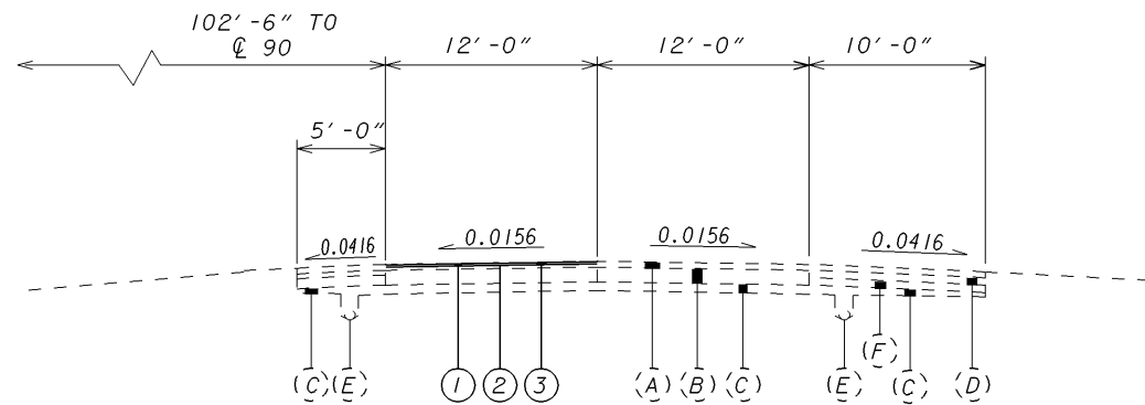
2 LANE NORMAL SECTION SLM 12.4 TO 14.63 (FOR LEFT LANES MIRROR ABOUT CL)
