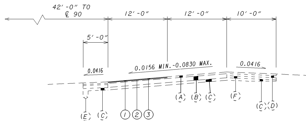
2 LANE SUPERELEVATED SECTION SLM 19.62 TO 20.57 (FOR LEFT LANES MIRROR ABOUT CL)
