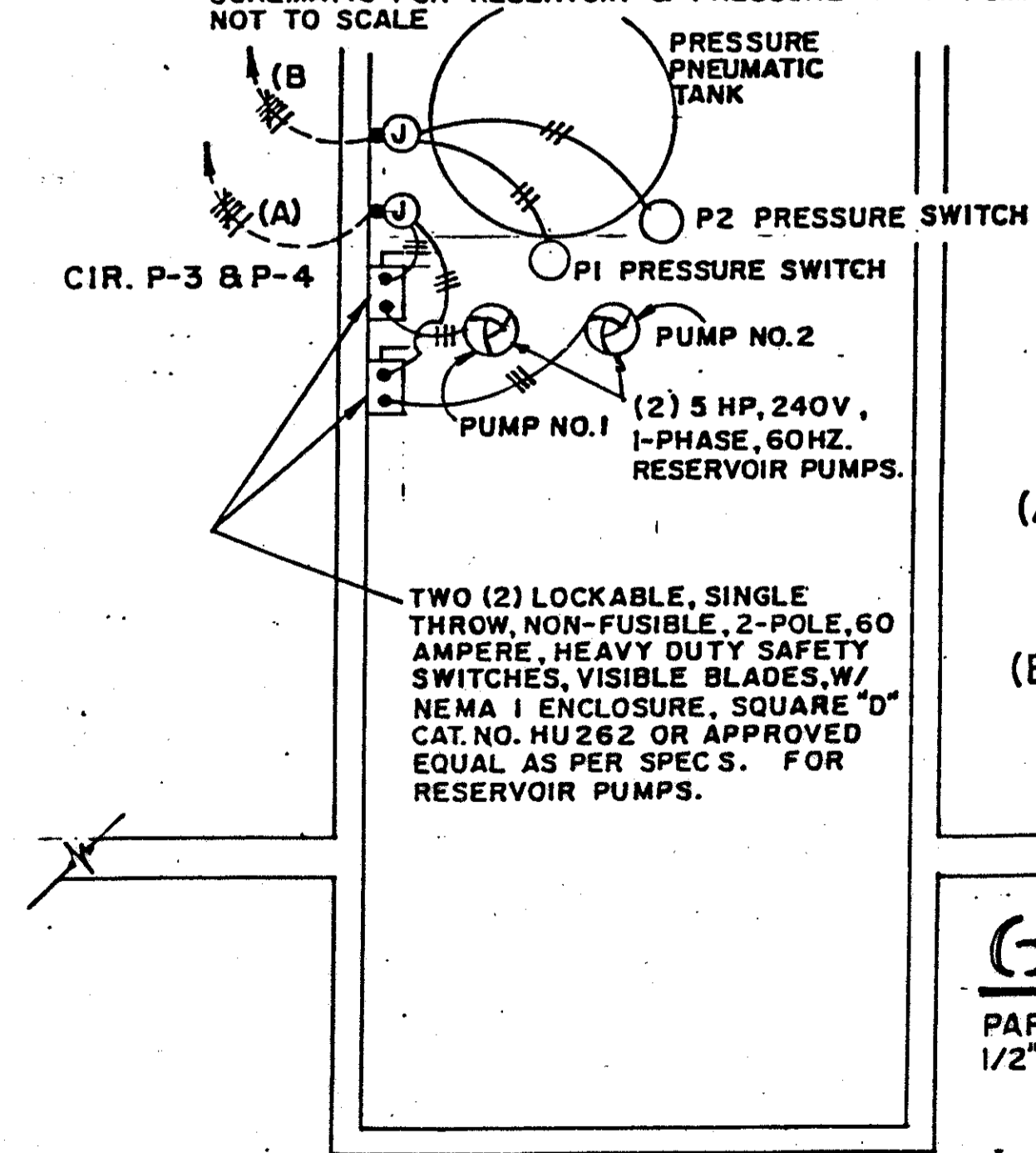
6G-03 SCHEMATIC FOR RESERVOIR & PRESSURE PUMP CONTROL NOT TO SCALE
