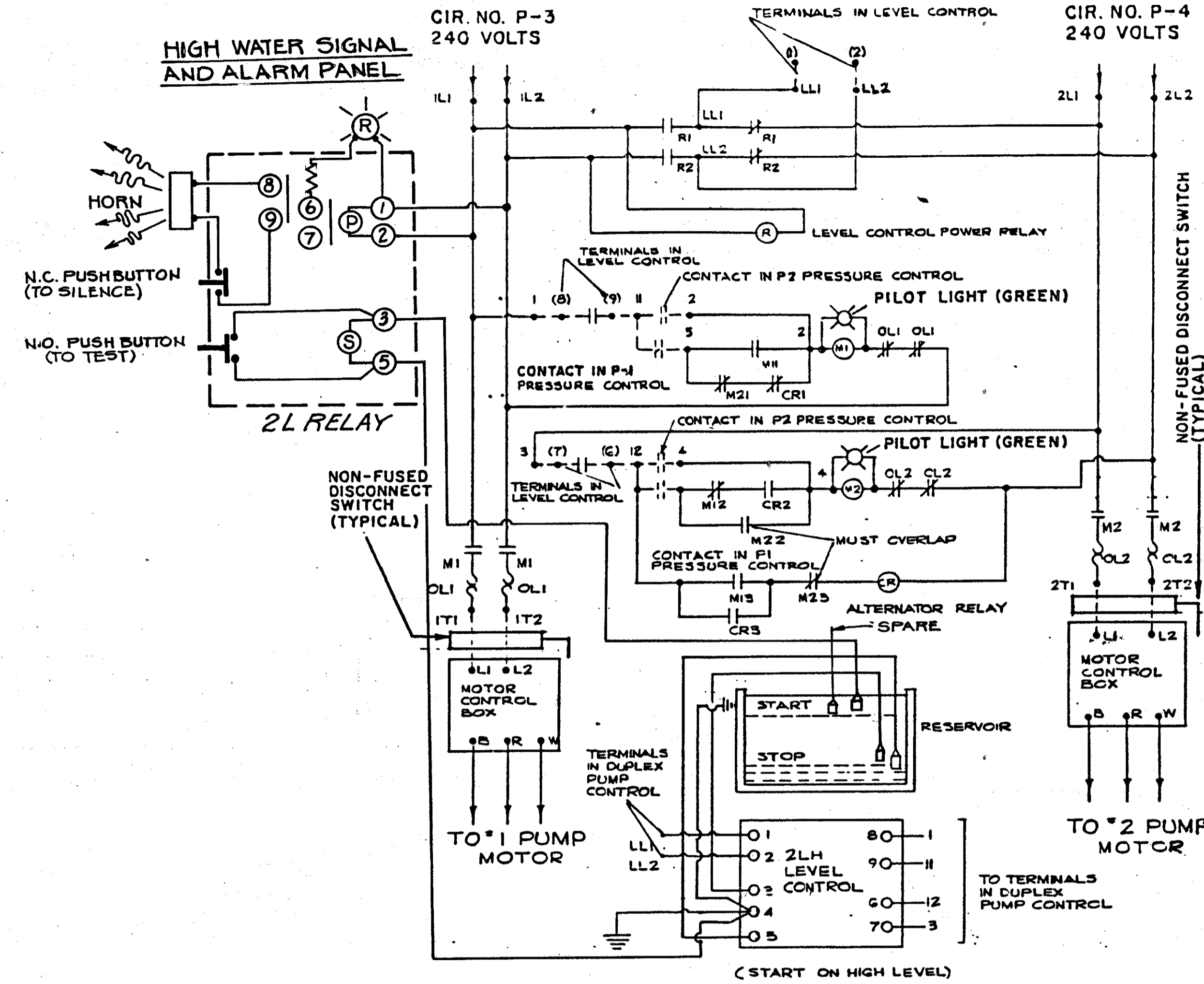
6G-03 SCHEMATIC FOR RESERVOIR & PRESSURE PUMP CONTROL NOT TO SCALE
