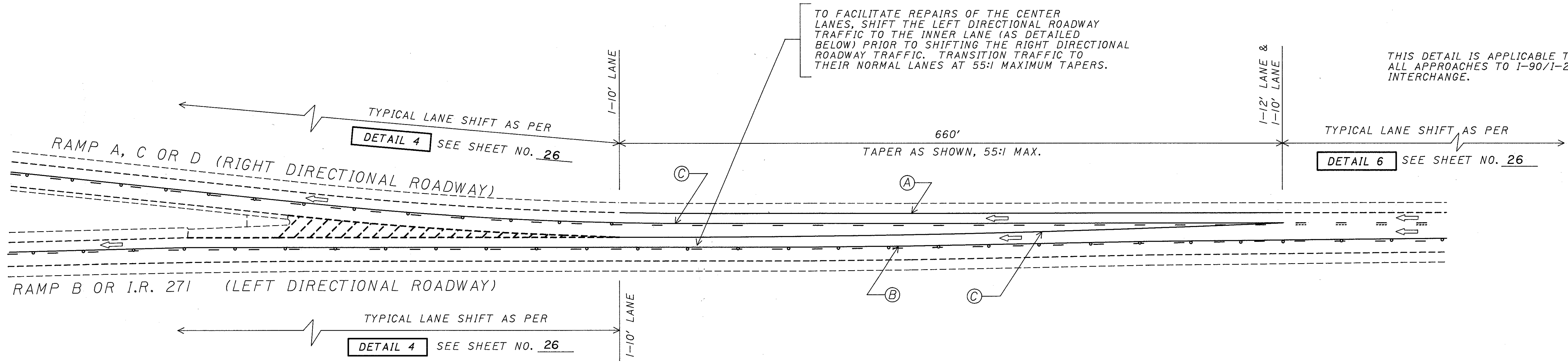
I.R. 271/I.R. 90 SPLIT PHASE I - LEFT LANE CLOSED
