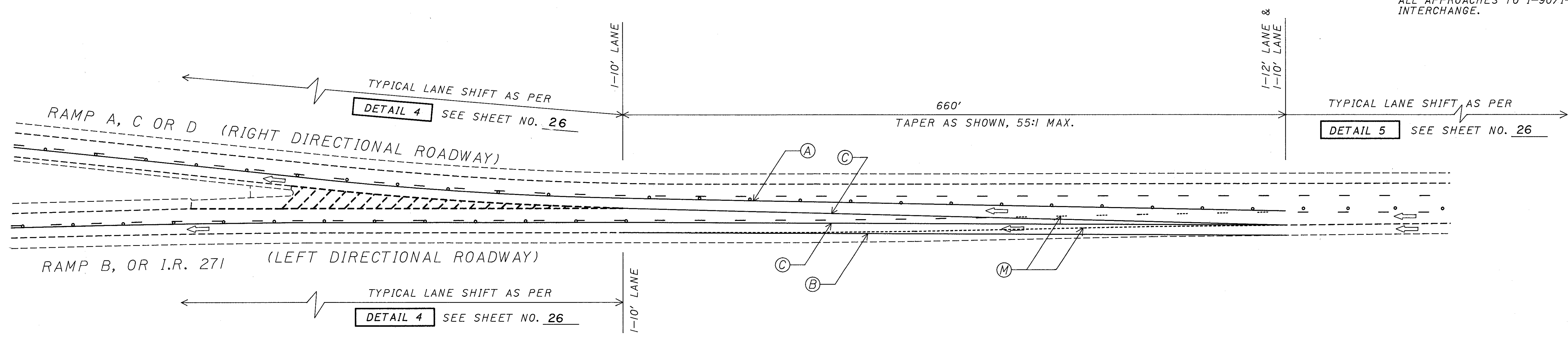
I.R. 271/I.R. 90 SPLIT PHASE I - LEFT LANE CLOSED
