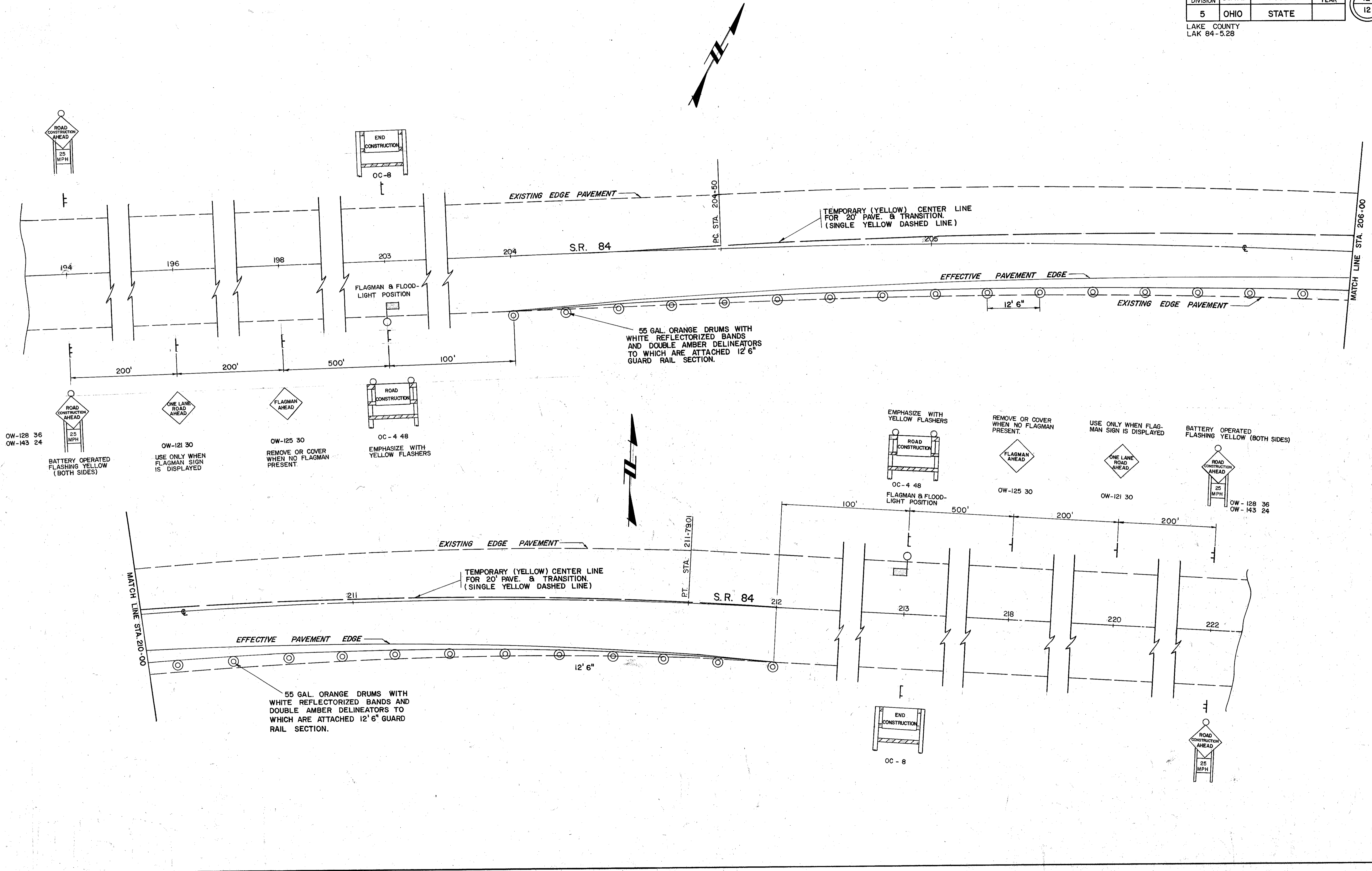
PLAN - TRAFFIC CONTROL DEVICES
