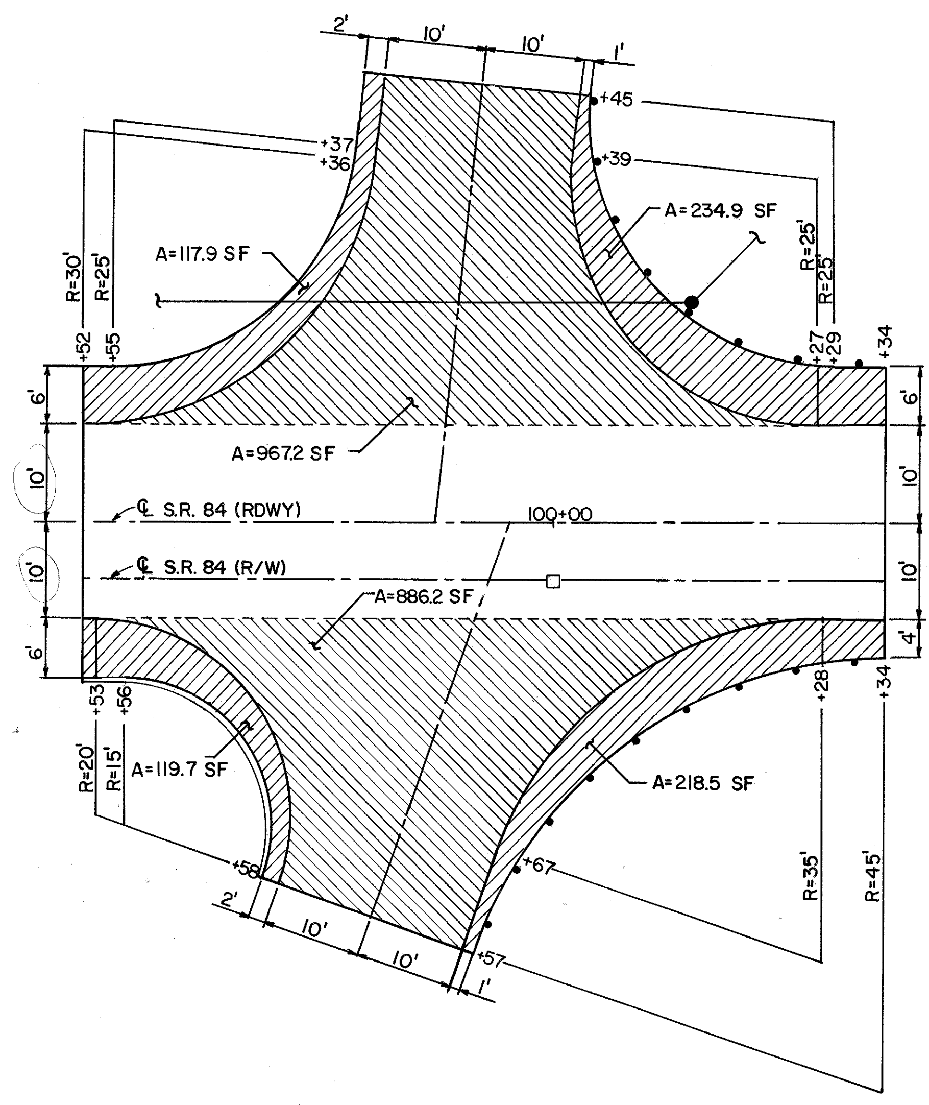
EXTRA AREA DETAIL INTERSECTION OF S.R. 84 & WOOD RD.
