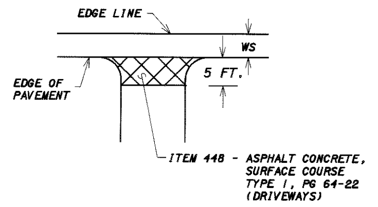
DRIVEWAY APRON DETAIL
