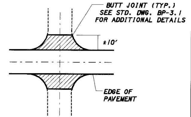
TYPICAL INTERSECTION DETAIL
