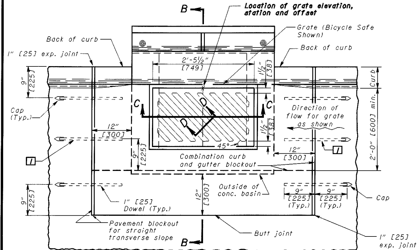
PLAN OF CATCH BASIN AND PAVEMENT JOINTS (For SECTIONS B-B and C-C, see Sht. 2/2)
