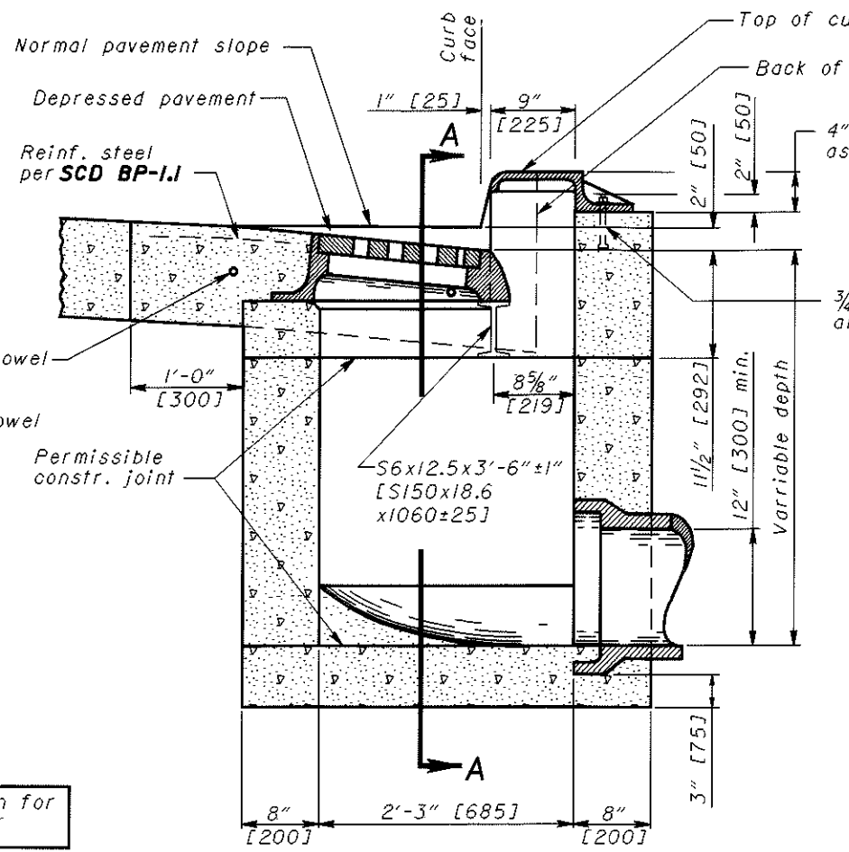
SECTION B-B WITH CURB (2" [50] DEPRESSION)
