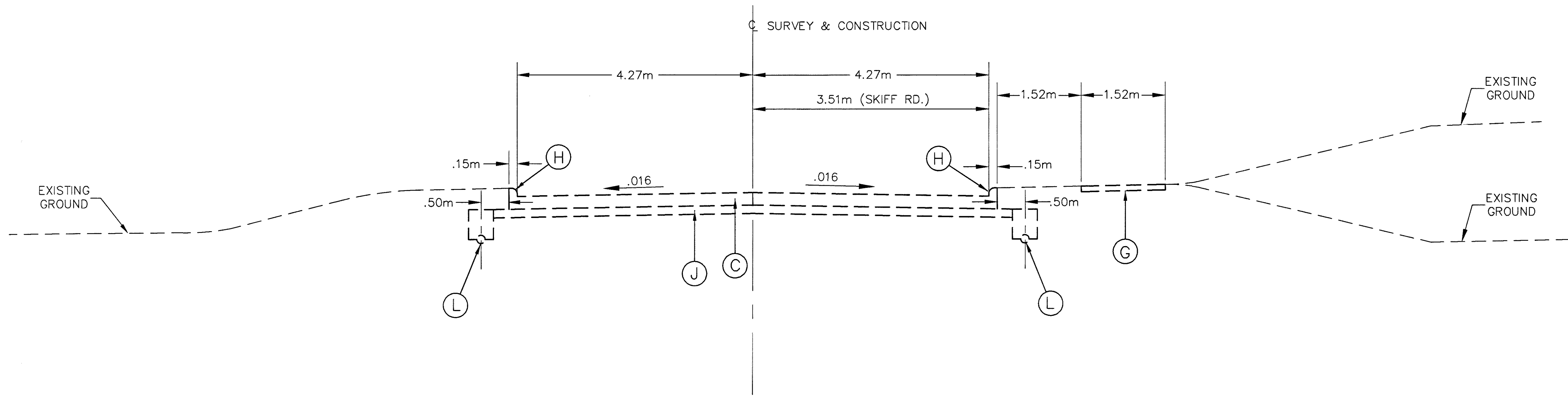
NORMAL SECTION BEN-HUR SERVICE ROAD SKIFF SERVICE ROAD FOR LEGEND, SEE SHEET NO.
