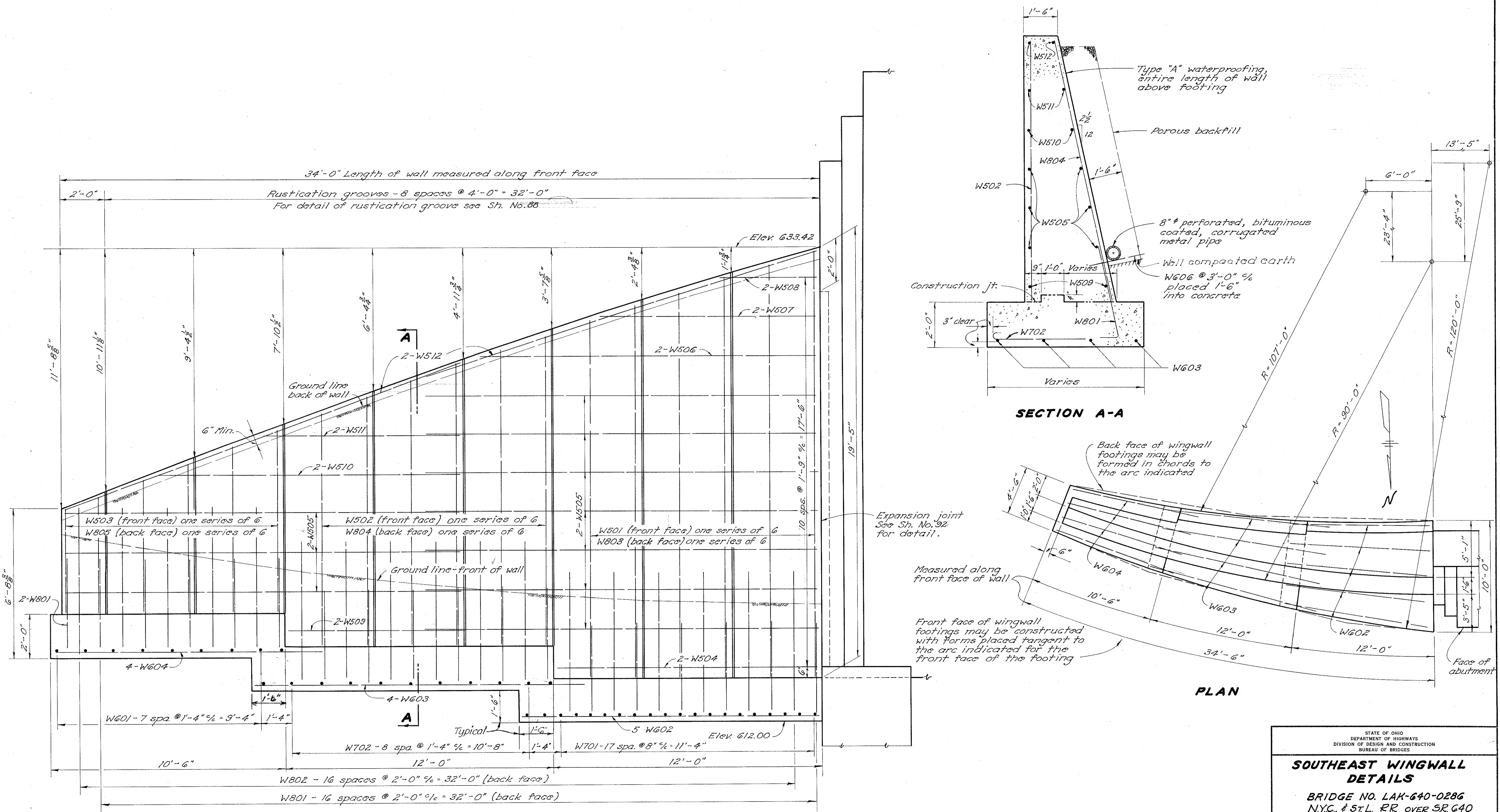
SOUTHEAST WINGWALL - DEVELOPED ALONG FRONT FACE OF WALL
