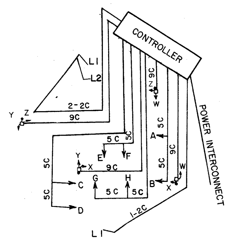
WIRING DIAGRAM
