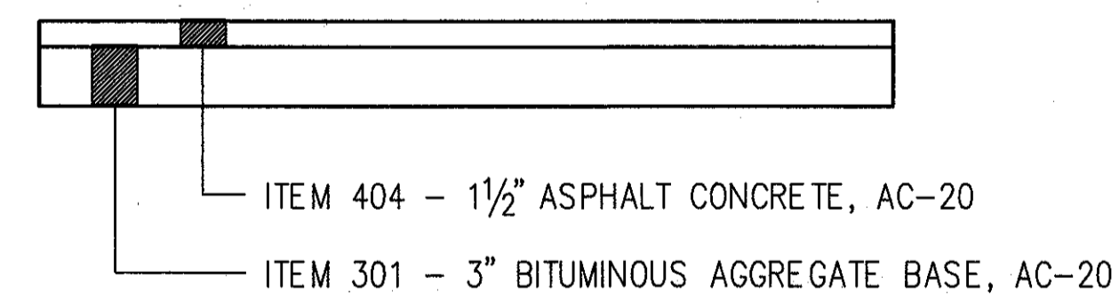
TYPE A DRIVE REPLACEMENT
