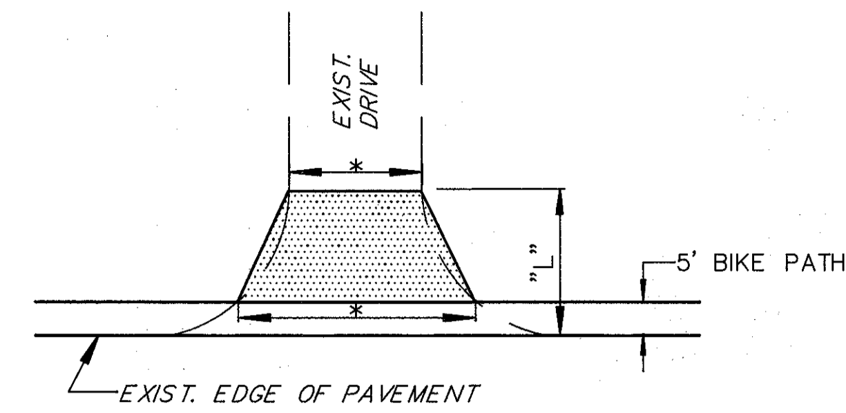
TYPE A DRIVE DETAILS
