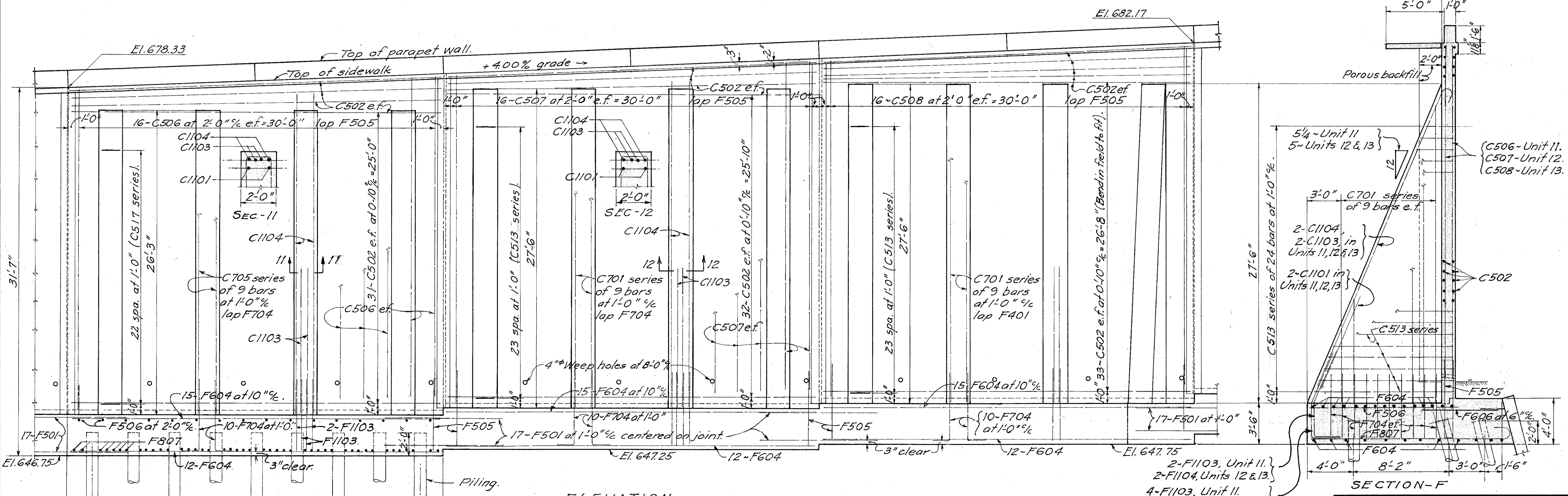
ELEVATION (Piling not shown in Units 12 & 13.)
