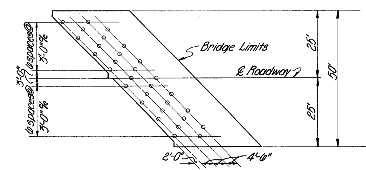
For additional details see Std. Dwg. AS-1-07 PLAN OF PAVEMENT JACKING HOLES
