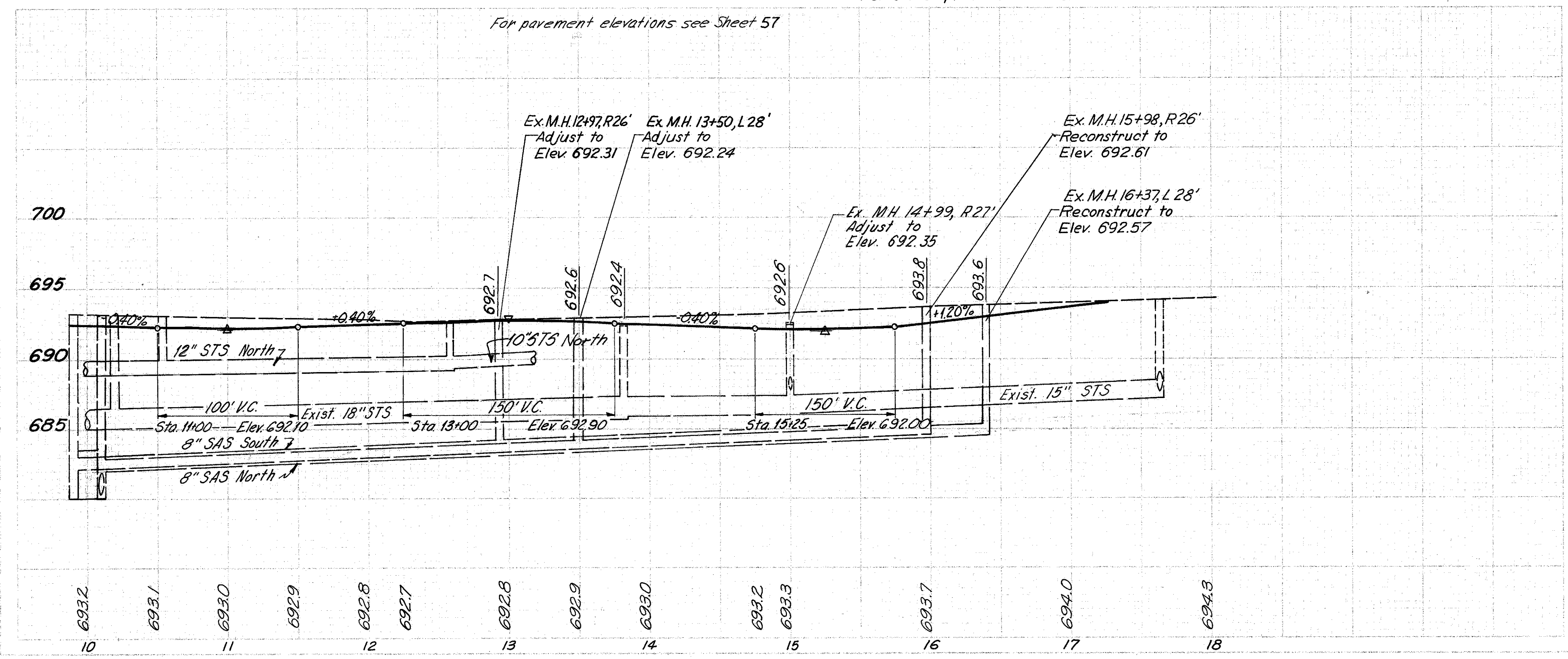
ADJACENT PAVEMENT SECTION MENTOR AVE.
