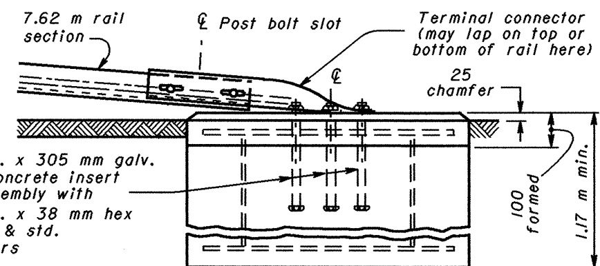
CONCRETE ANCHOR
