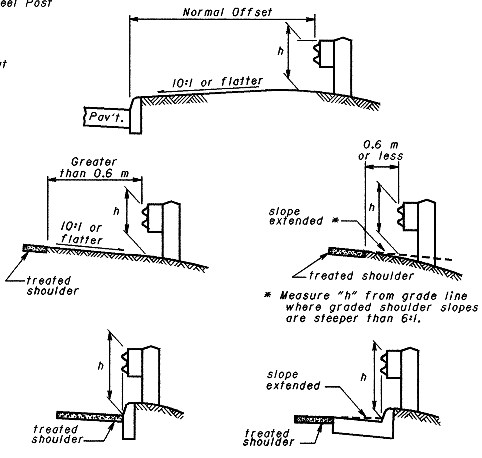
MEASURING GUARDRAIL HEIGHT
