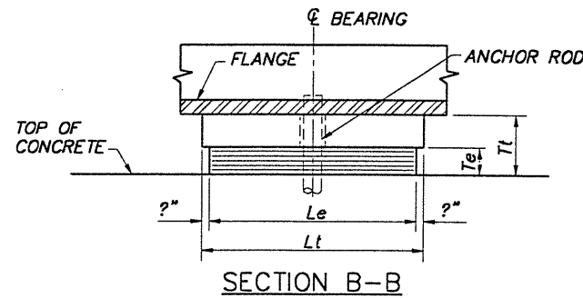
SECTION B-B LAMINATED ELASTOMERIC FIXED BEARING AT PIER 2
