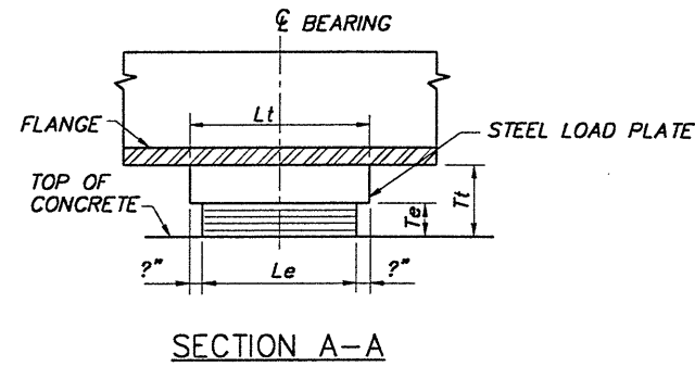
SECTION A-A LAMINATED ELASTOMERIC EXPANSION BEARING AT PIER 1
