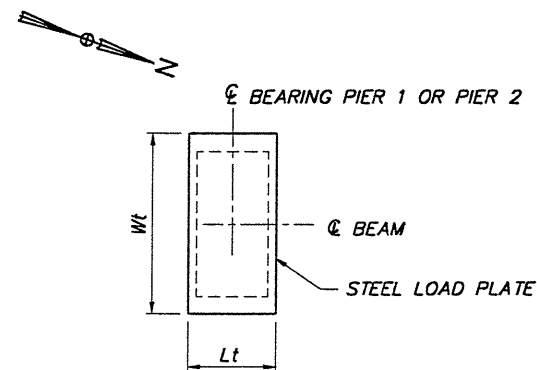
BEARING ORIENTATION PLAN
