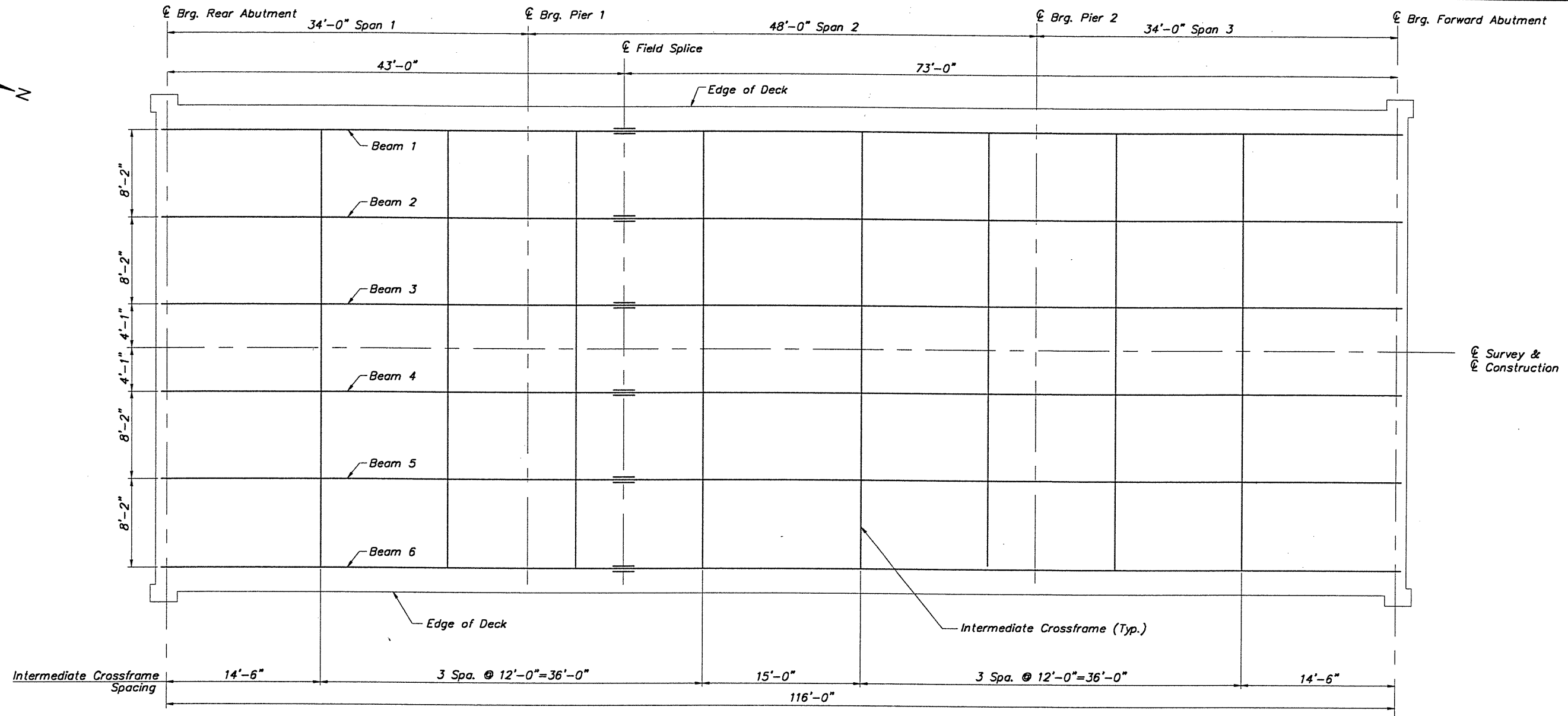
STEEL FRAMING PLAN
