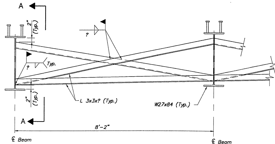
INTERMEDIATE CROSSFRAME DETAIL
