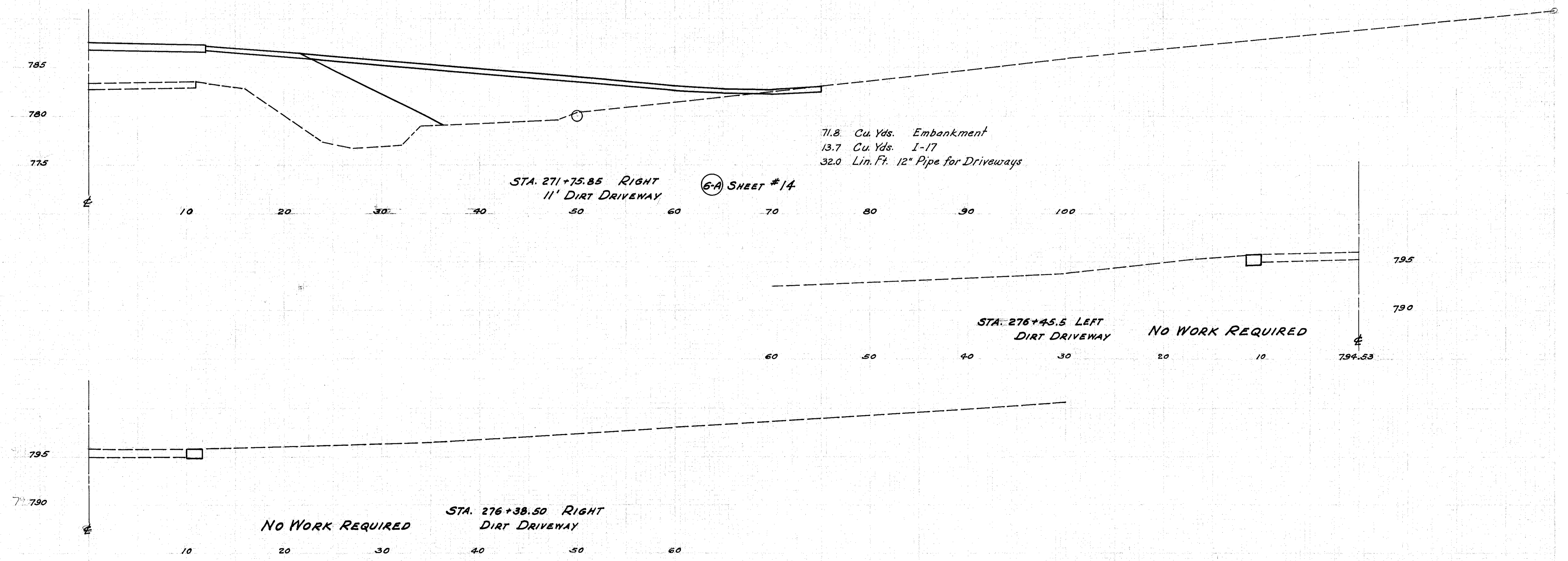
DRIVEWAY PROFILES STA 276+38.50-STA 271+7585
