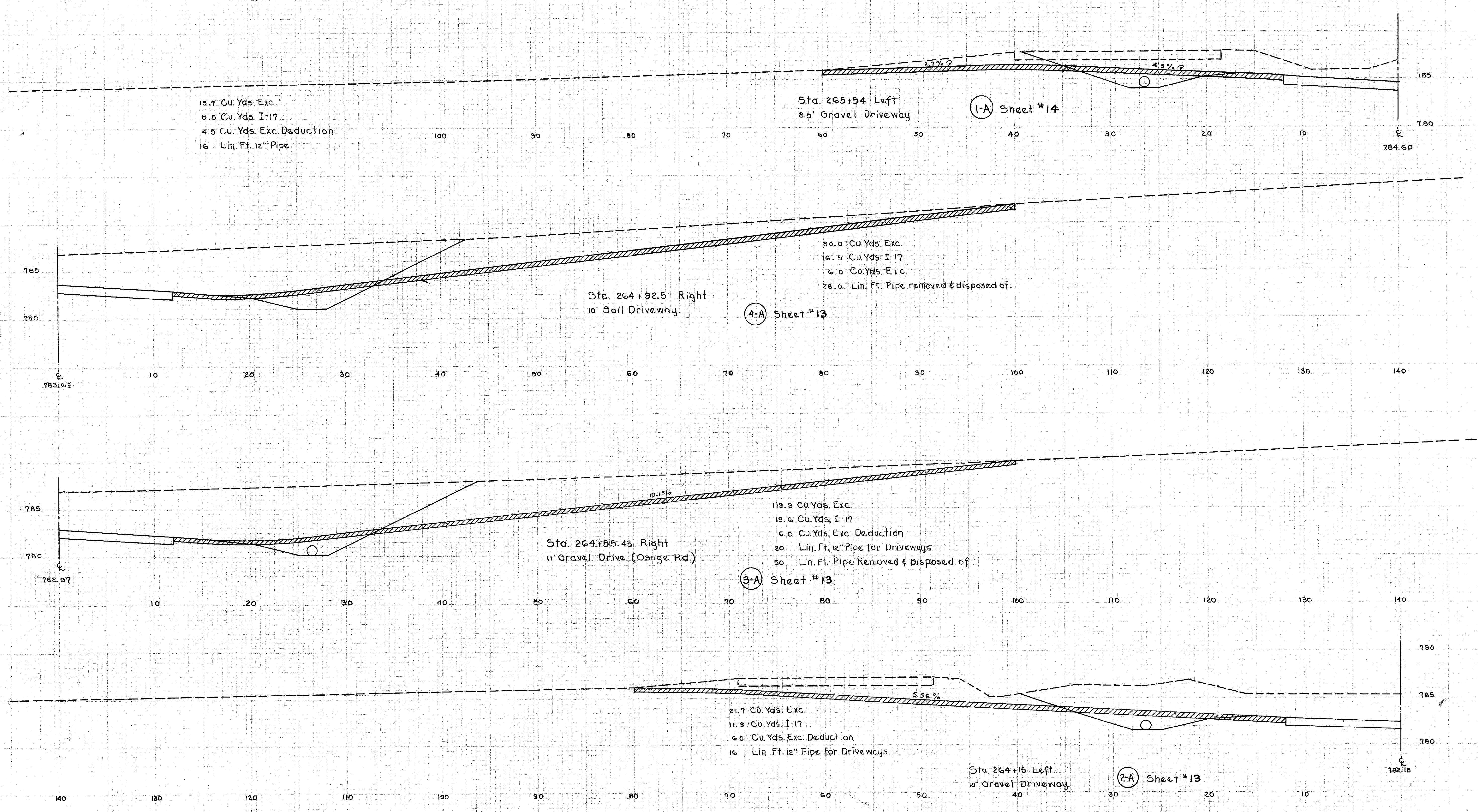
DRIVEWAY PROFILES—STA 264+15— STA 265+54
