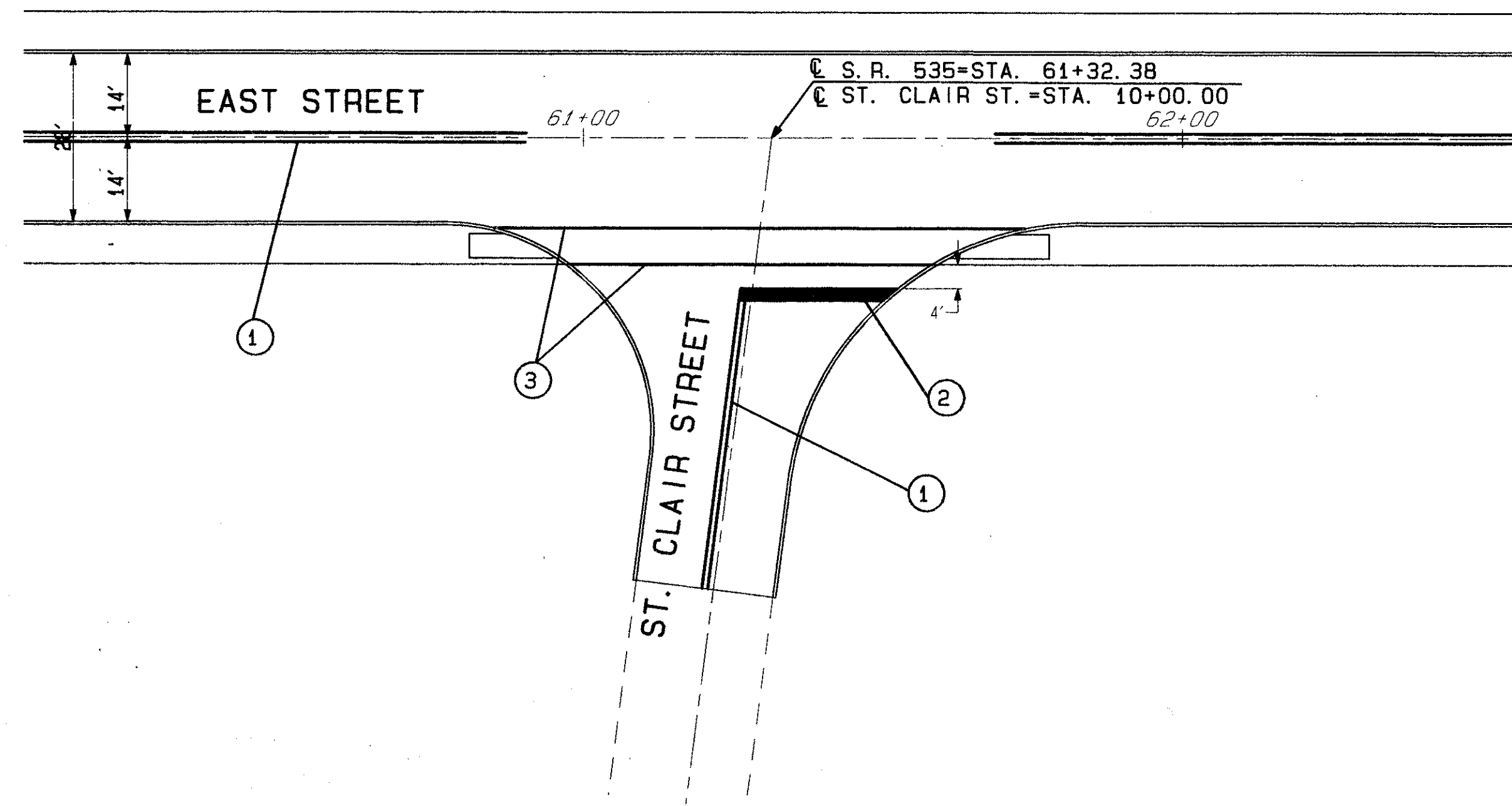
NON-SIGNALIZED "T" INTERSECTION ST. CLAIR STREET
