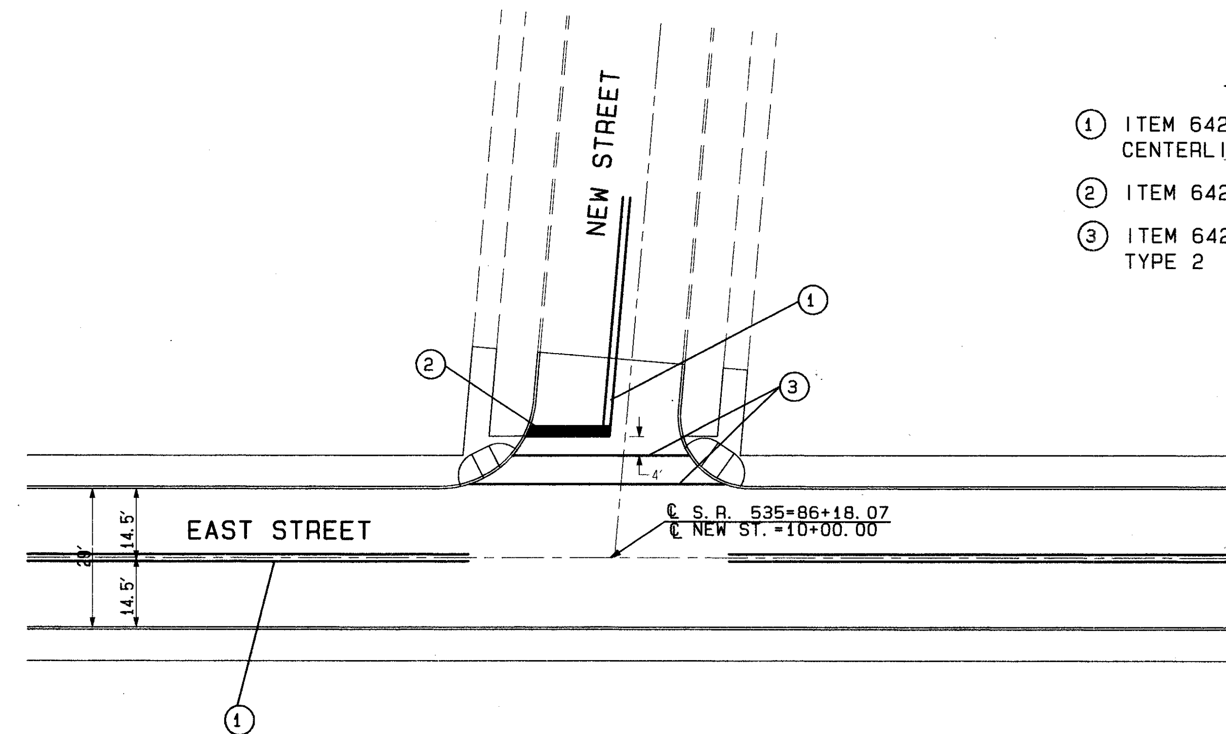
NON-SIGNALIZED "T" INTERSECTION NEW STREET
