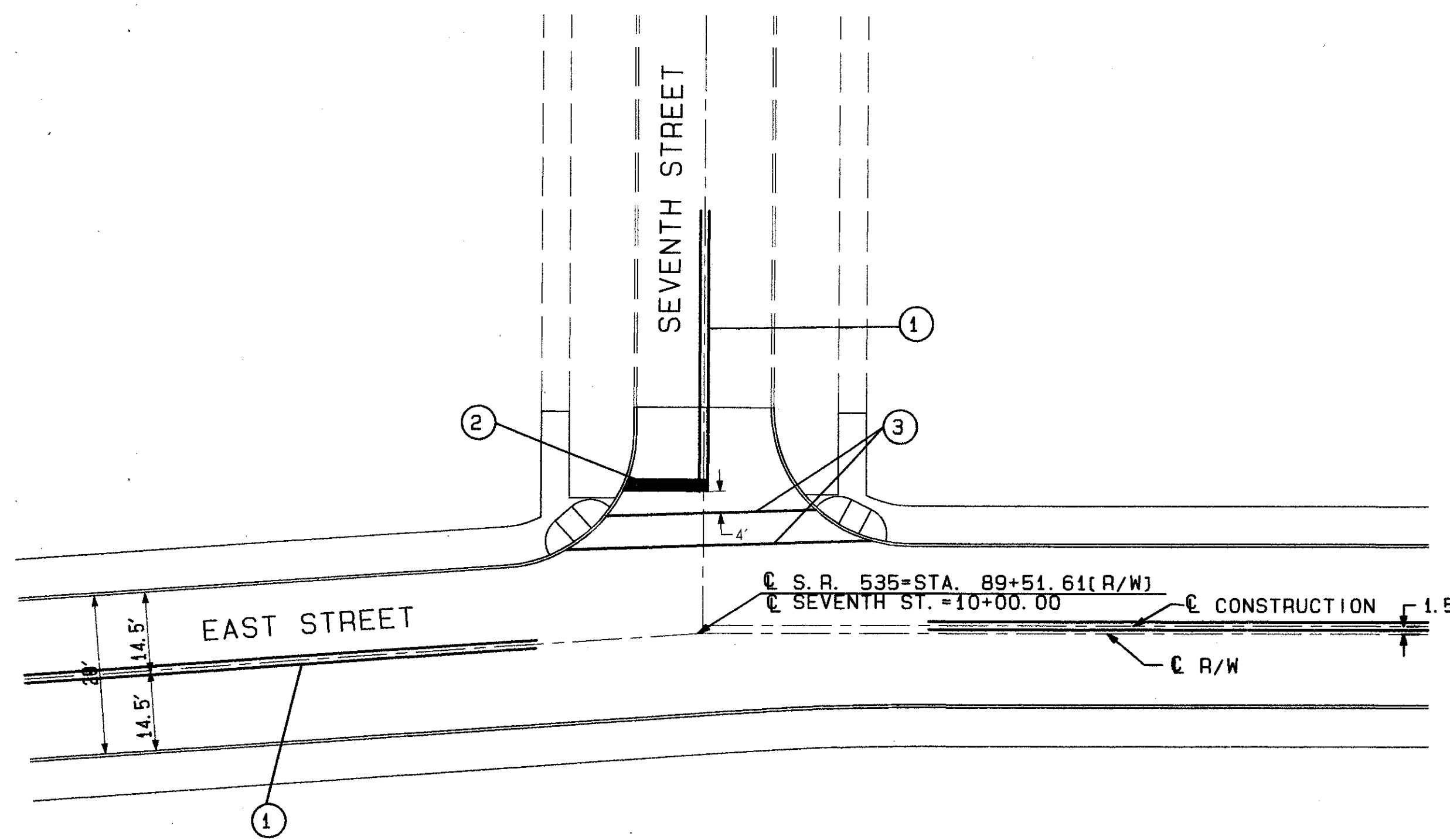
NON-SIGNALIZED "T" INTERSECTION SEVENTH STREET
