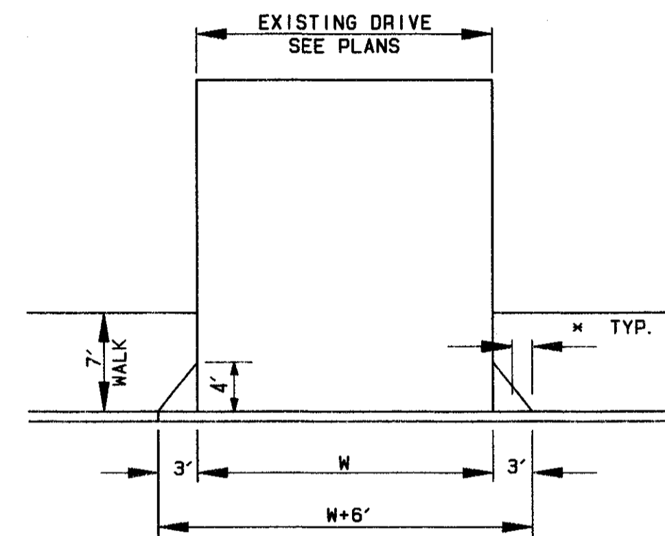
TYPICAL DRIVE DETAIL
