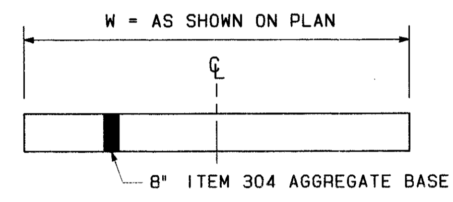
RESIDENTIAL STONE DRIVE
