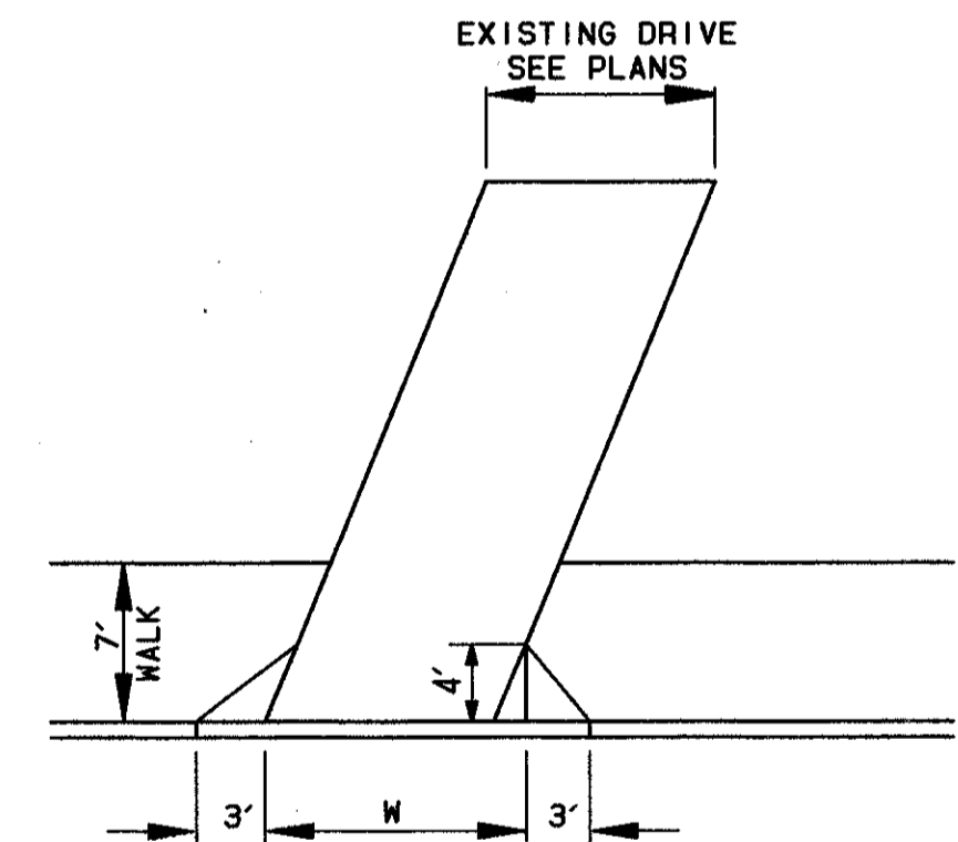
TYPICAL DRIVE DETAIL
