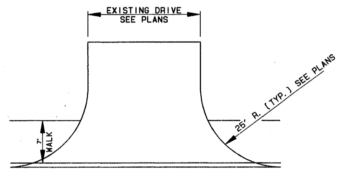
TYPICAL DRIVE DETAIL
