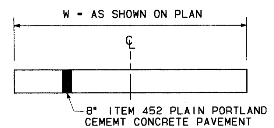
COMMERCIAL CONCRETE DRIVE
