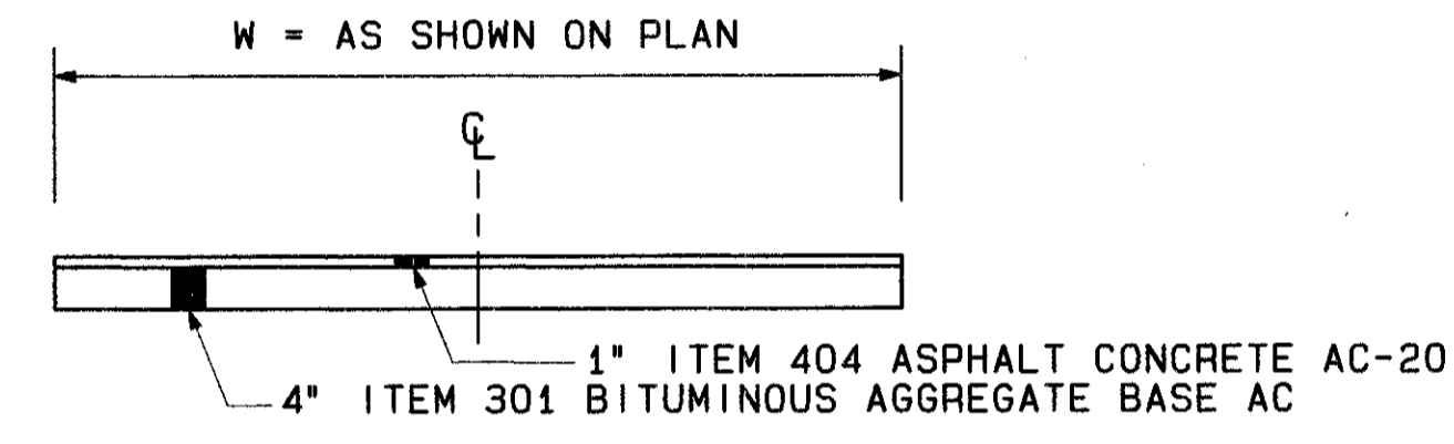
RESIDENTIAL ASPHALT DRIVE
