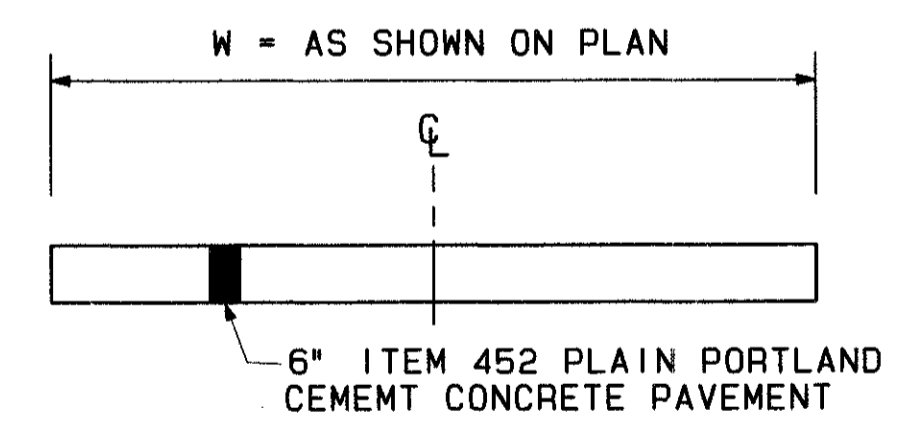
RESIDENTIAL CONCRETE DRIVE
