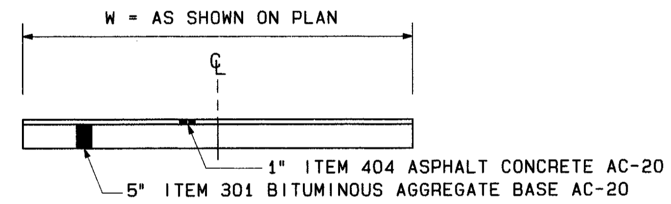
COMMERCIAL ASPHALT DRIVE
