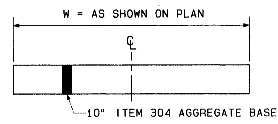
COMMERCIAL STONE DRIVE
