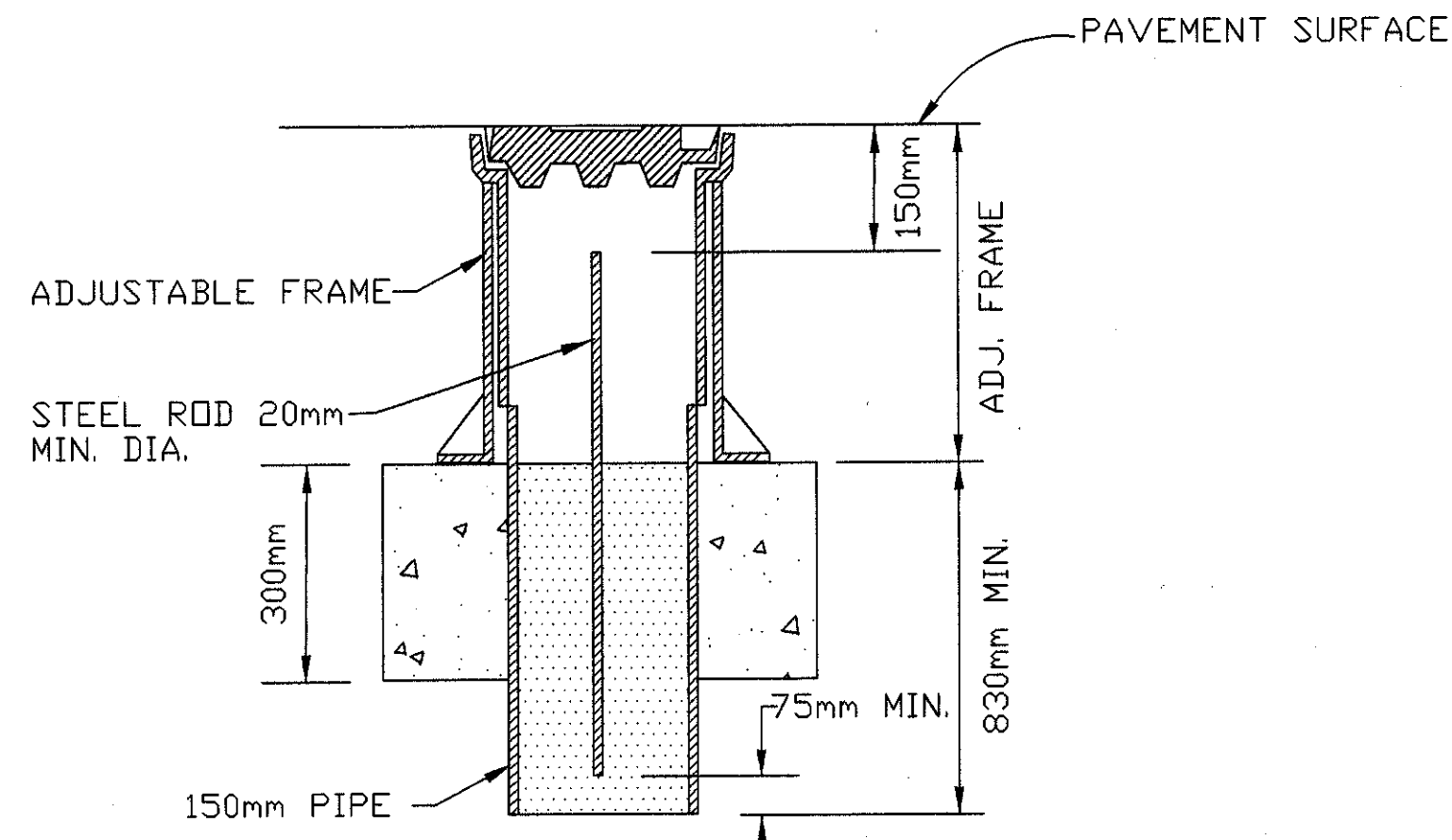
SIDE VIEW ADJUSTABLE CENTERLINE MONUMENT DETAILS
