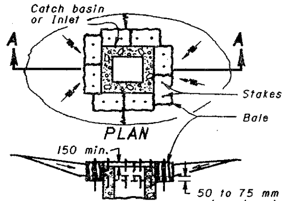
SECTION A-A BALE INLET FILTER
