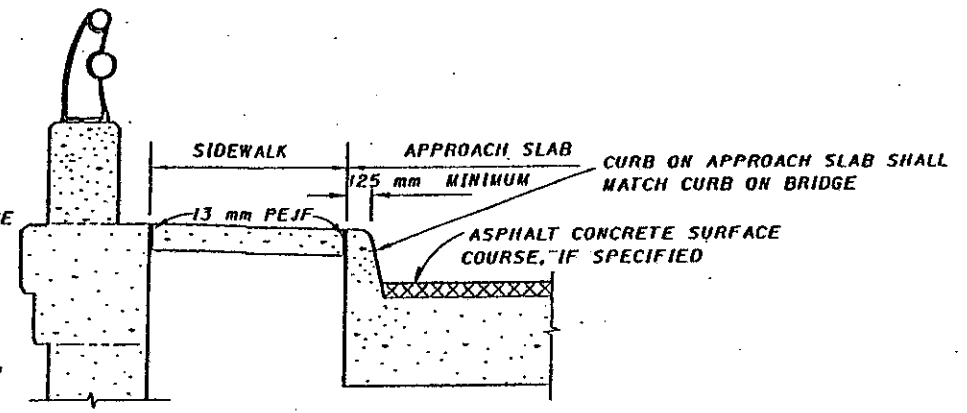
SECTION C-C
