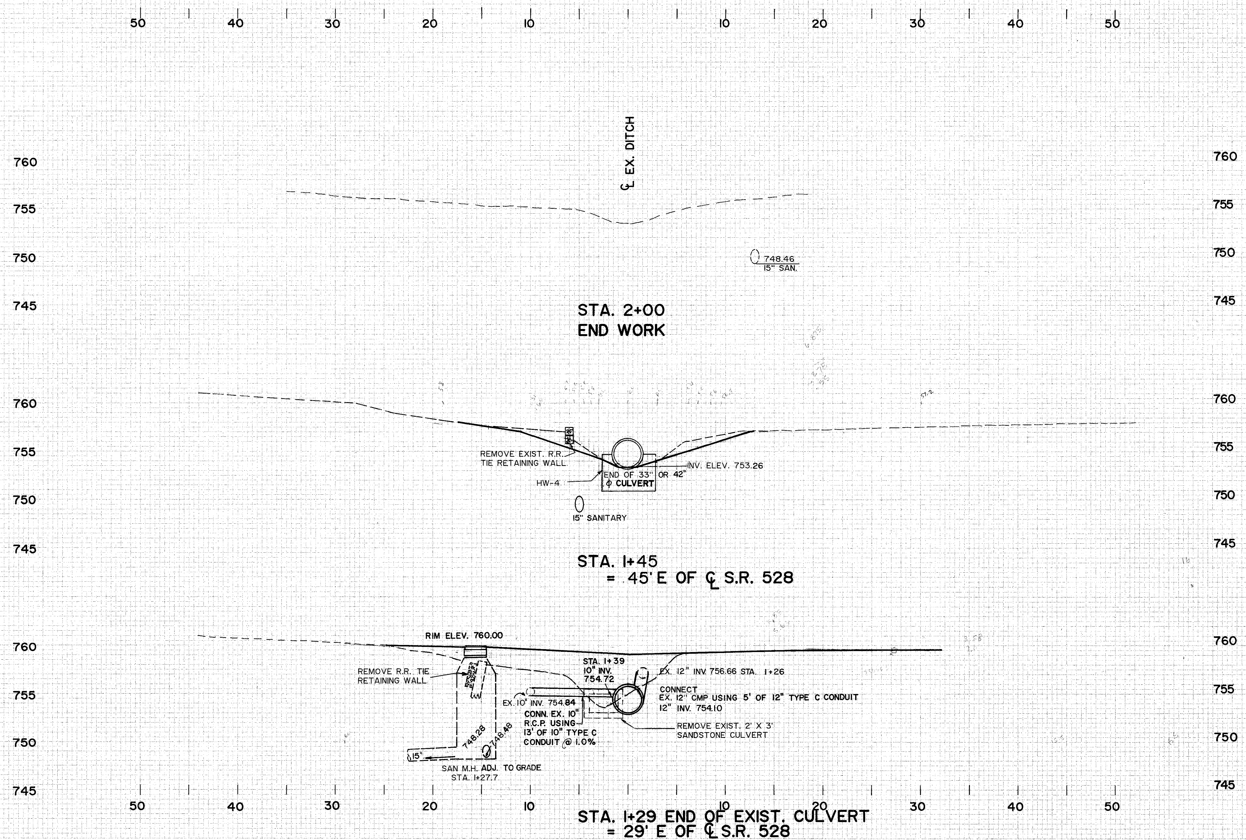
CULVERT CROSS SECTIONS
