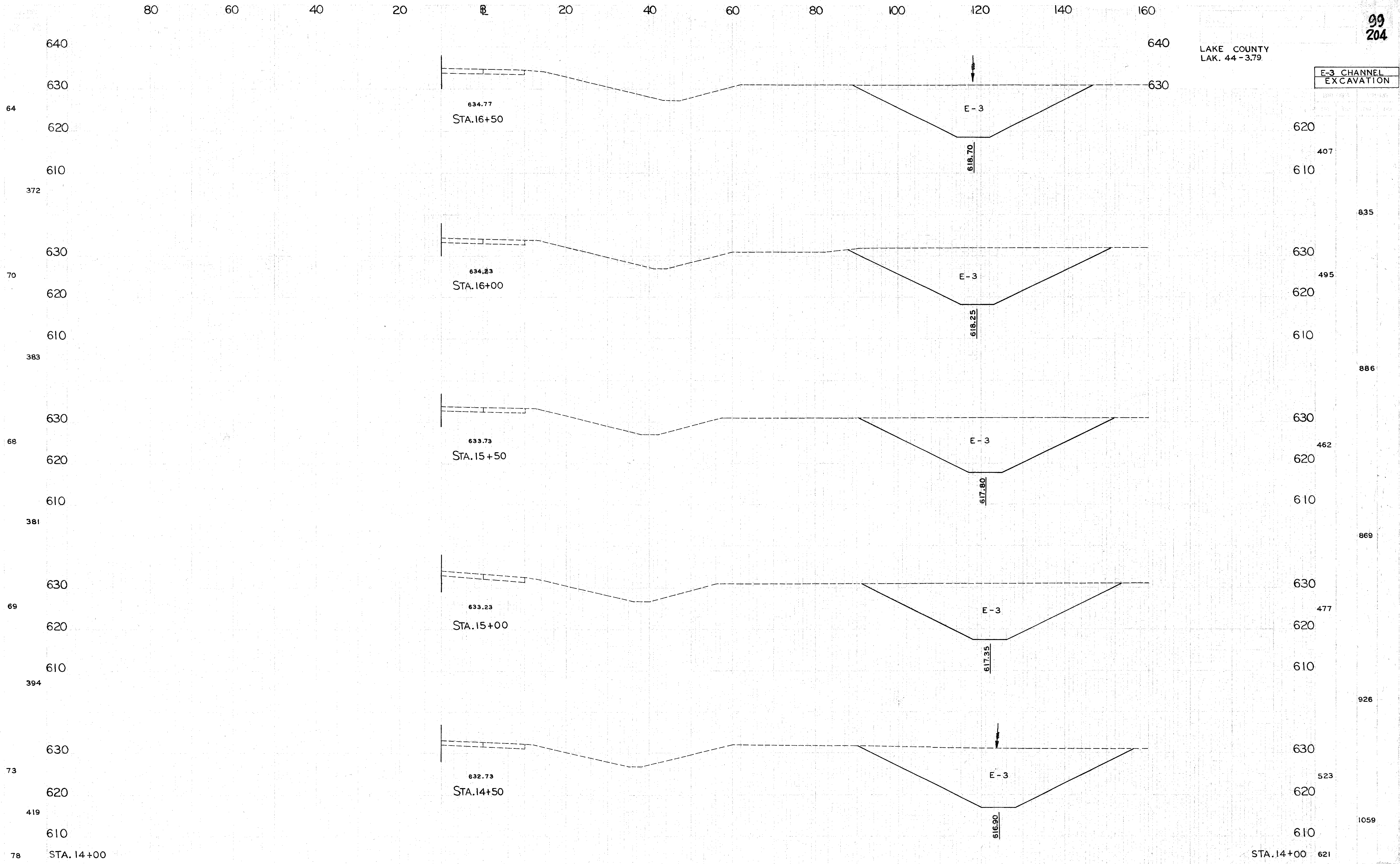
RAMP "F" STA.14+50 TO STA.16+50
