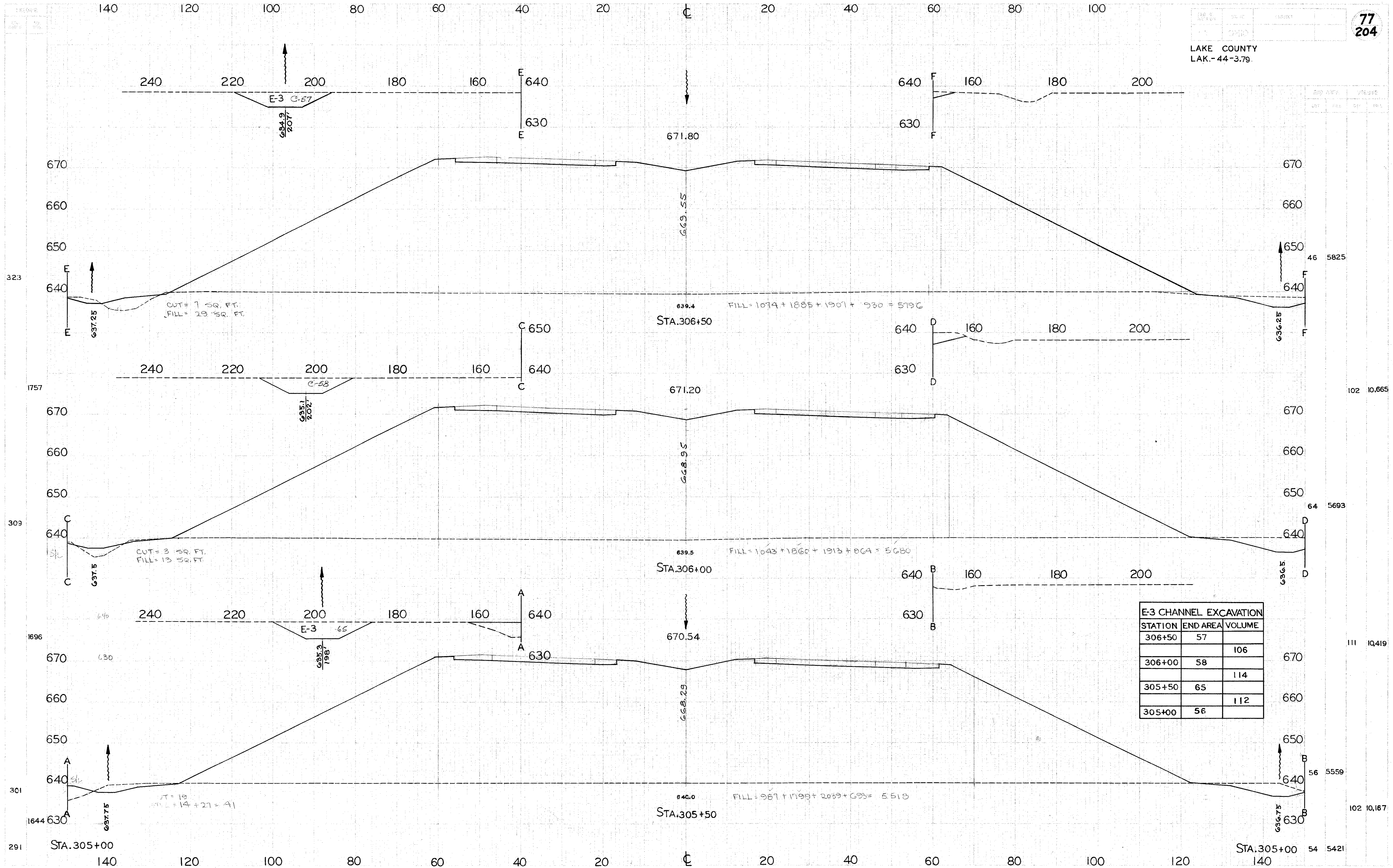
CROSS SECTIONS STA.305+50 TO STA.306+50
