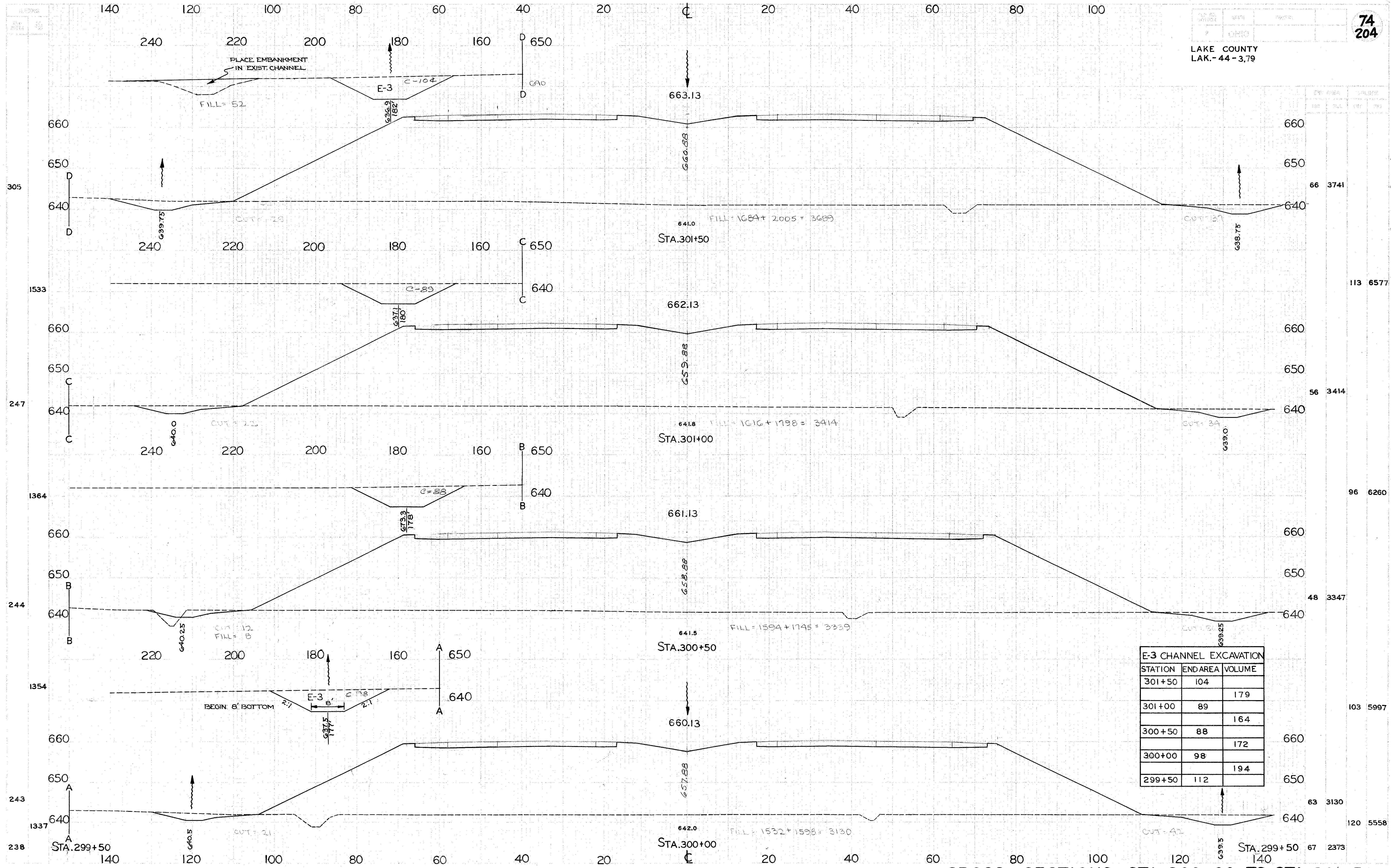
CROSS SECTIONS STA.300+00 TO STA.301+50
