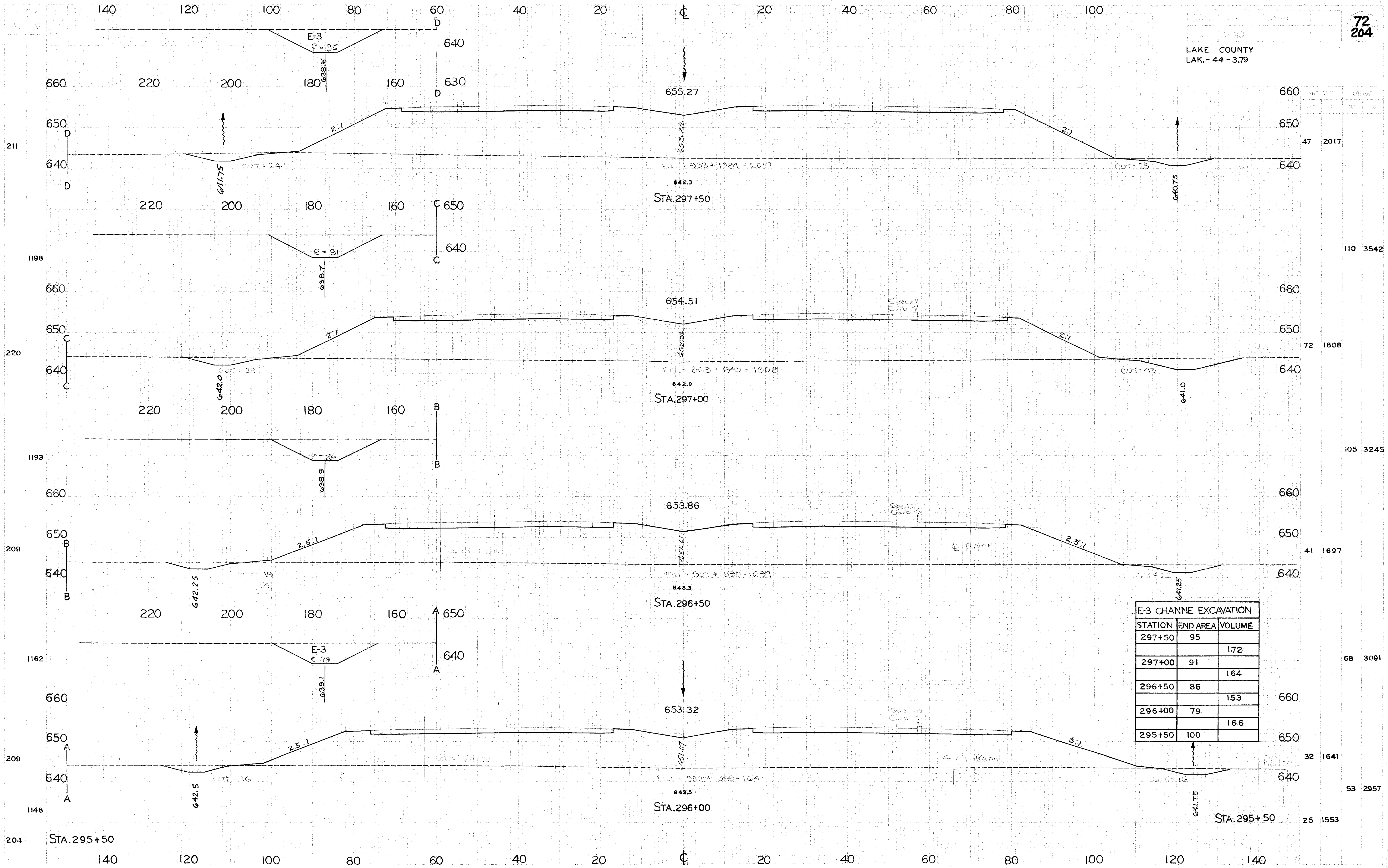
CROSS SECTIONS STA.296+00 TO STA.297+50
